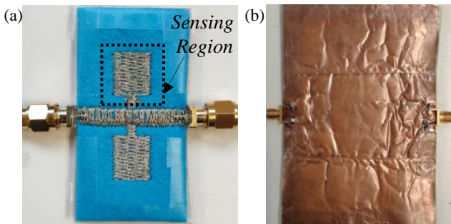
Fig. 5. Top (a) and bottom (b) views of the fabricated textile microwave frequency-splitting sensor. The sensing region is indicated.
