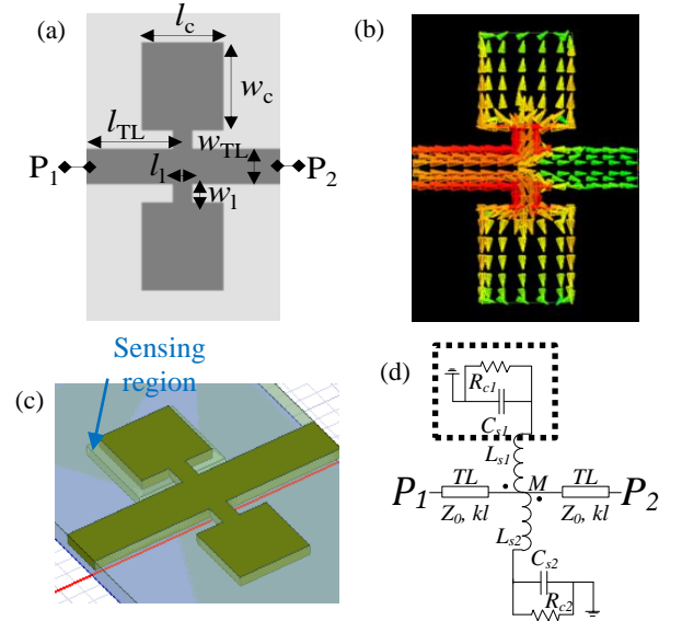
Fig.1. 2D Layout (a), electric field distribution at the resonance frequency ( f_0 ) of the coupled SIRs (b), 3D HFSS layout view (c), and equivalent circuit model (d) of the proposed differential microwave sensor. The ground plane is depicted in soft grey color. The relevant dimensions are indicated.
