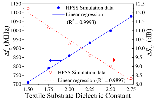
Fig.4. Representation of simulated \Delta f_z = f_2 - f_1 and \Delta S_{21} = S_{21min,f_2} - S_{21min,f_1} as a function of the dielectric properties of the considered textile substrate for the implementation of real differential sensor. Note that the horizontal axis corresponds to the real part of the complex dielectric constant of the MUT. The corresponding values of the imaginary part can be deduced from the insets of Fig. 3.
