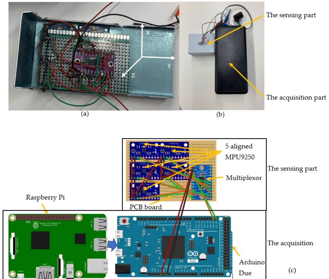
Figure 1. LARA elements: (a) the adjustments and wire connections of the sensing part, (b) the sensing and acquisition part, and (c) LARA in detail.
