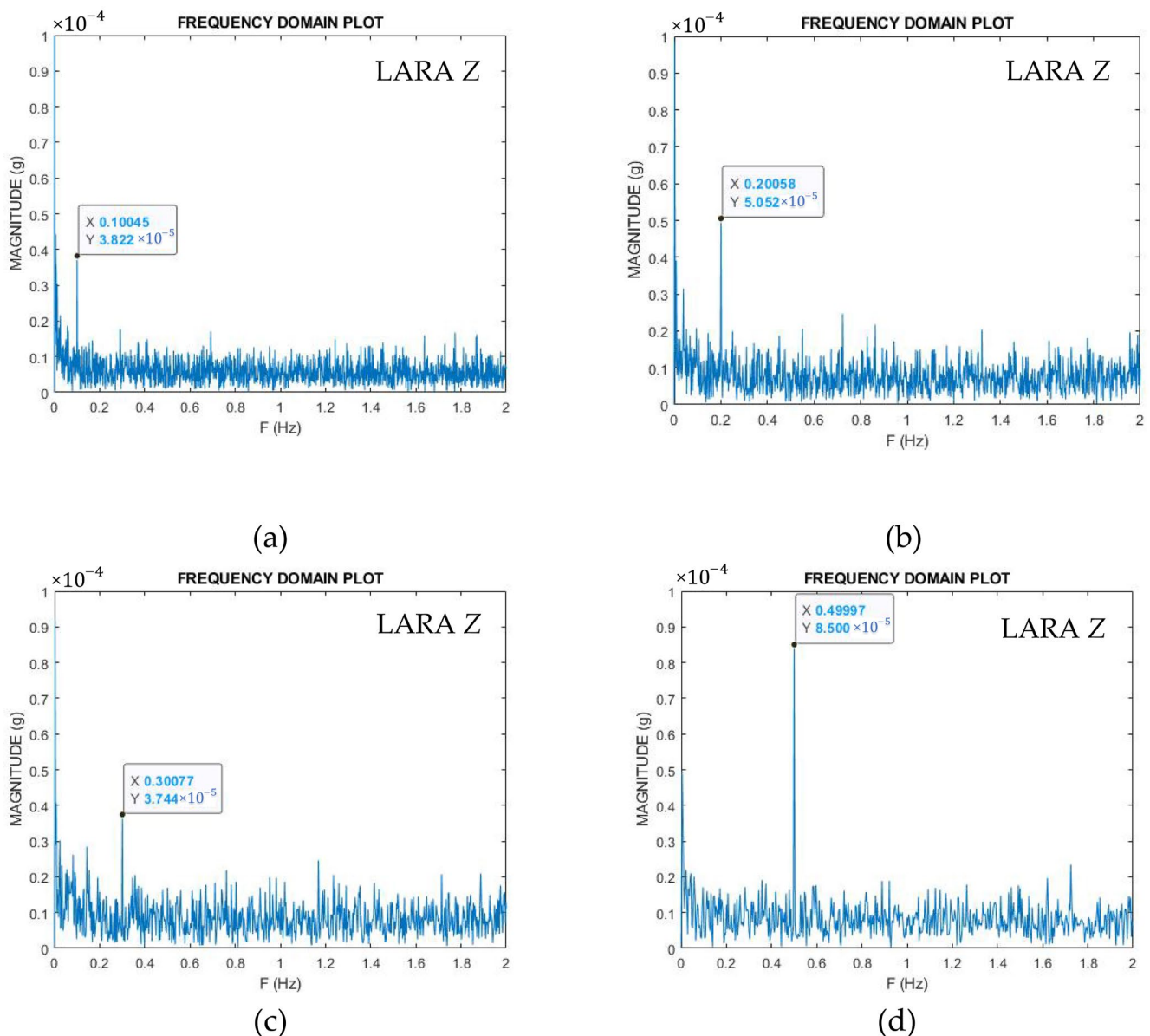
Figure 5. FFT representation of the low-frequency signals: (a) 0.1 Hz, (b) 0.2 Hz, (c) 0.3 Hz, and (d) 0.5 Hz.
