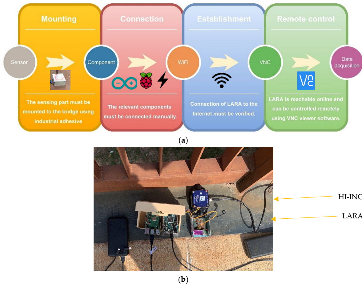
Figure 11. Mounting the sensors to the mid span of the bridge under study: (a) mounting diagram of LARA to the bridge and (b) photo of LARA and HI-INC sensor mounted on a footbridge in Barcelona.
