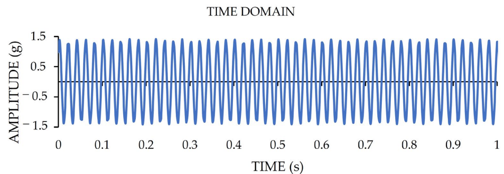
Figure 8. The time-domain presentation of a vibration acquisition with RMS value of one g by LARA.
