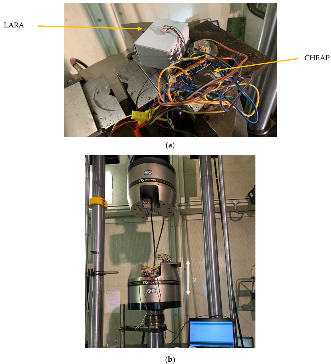
Figure 4. Laboratory validation of LARA: (a) mounting CHEAP and LARA to the shaking part of the jack, and (b) the used vibrating platform (INSTRON 8803).
