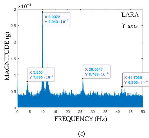
Figure 12. Eigenfrequency analysis of a footbridge using LARA for (a) vertical, (b) longitudinal, and (c) transversal directions of the footbridge.
