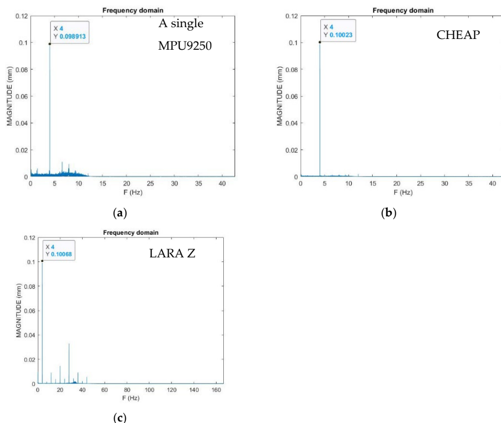
Figure 7. Displacement report of the accelerometers: (a) MPU9250, (b) CHEAP, and (c) LARA.
