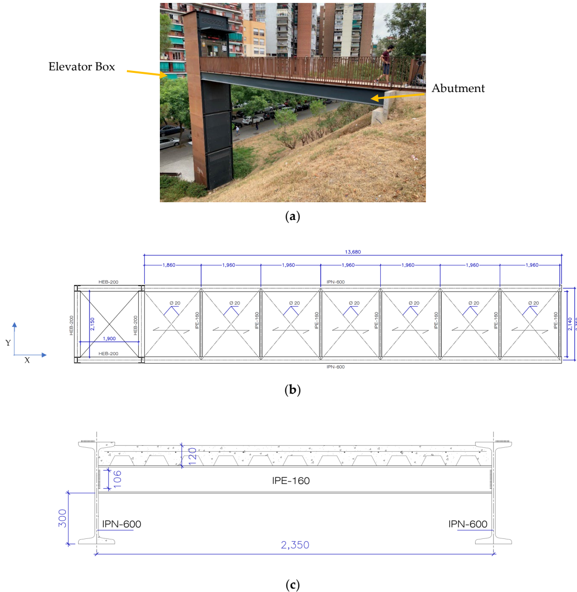
Figure 10. (a) A picture of the pass way, (b) plan of the bridge, and (c) section of the pass way bridge (all units are in mm).
