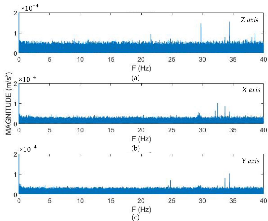
Figure 3. Frequency domain diagrams of LARA for: (a) z , (b) x , and (c) y -axis.
