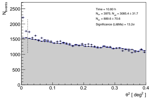
Fig. 4 Distribution of the squared angular distance between the nominal source position and the reconstructed arrival direction of events (black crosses) and the estimated background (gray shaded area). Vertical dashed line represents the angular cut below which the number of background and excess events as well as the statistical significance of the detection are given (inset panel).
