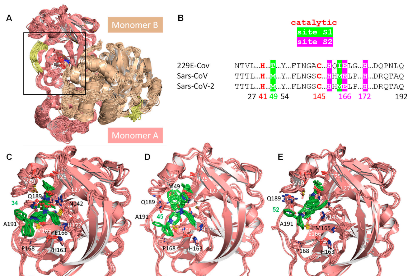
Figure 4. Ribbons representation of chymotrypsin-like protease M P ro from SARS-CoV-2. (A) Overlay of 30 snapshots taken at regular intervals from the unrestrained molecular dynamics simulation in water lasting 150 ns. Each monomer is displayed in a different color and the 187 Asp-Ala 193 stretch is highlighted in yellow. (B) Alignment of active site amino acids from HCoV-229E, SARS-CoV and SARS-CoV-2 M P ro enzymes that are proposed to have a direct bearing on ligand binding, as discussed in the text. (C–E) Theoretical models of one monomer of SARS-CoV-2 M P ro (ribbons with C atoms colored in pink) in complex with compound 34 (C) , 45 (D) and 52 (E) ; the region displayed corresponds to the boxed area in (A) . Ligands are shown as sticks with carbon atoms colored in green. Each set of five superposed structures represents a conformational ensemble made up of snapshots taken every 5 ns from the post-equilibrated 75–100 ns interval of the simulated trajectories and then cooled down to 273 K and energy minimized. For reference, some of the residues closest to the ligands have been labeled. Water molecules are not displayed for enhanced clarity.
