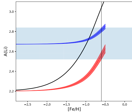
Figure 16. The Li evolution in the SMC assuming the nova yields derived in this paper starting from two different Li initial values: in red the Spite plateau and in blue the CMB + BBN nucleosynthesis. The two curves for each initial lithium abundance and the derived nova yields with their error are shown by shaded regions. The model include astration as well as spallation nucleosynthesis and a modest AGB contribution. The present Li abundance measured in the ISM of SMC derived by Howk et al. (2012) with \pm 1\sigma error is shown with the shaded horizontal band. Finally, the black curve shows the Li evolution derived when a chemical evolution of the SMC but with a Li-yield typical of our Galaxy, namely a factor 4 higher than of the SMC, is considered (Cescutti & Molaro 2019). Note how much the expected value for A(\text{Li}) would be off with respect to the present Li abundance value in the SMC if we consider MW-like yields.
