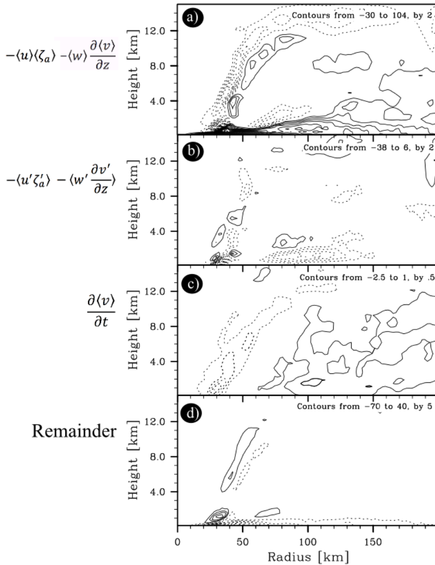
Figure 2. Two-hour average of the terms in the mean tangential velocity tendency equation, centered around hr 23 from the mesoscale simulation of TM08. The terms show are a) the combined contribution of the mean radial vorticity flux and the mean vertical advection of mean tangential momentum, b) the combined contribution of the perturbation radial eddy vorticity flux and the perturbation vertical advection of perturbation tangential momentum, c) the local time rate of change of mean tangential velocity, and d) the mean remainder, estimated as the difference between the third row and the sum of the first two rows. For clarity, contours are shown every 2 \text{ m s}^{-1} \text{ hr}^{-1} in panels a) and b), 0.5 \text{ m s}^{-1} \text{ hr}^{-1} in panel c) and 5 \text{ m s}^{-1} \text{ hr}^{-1} in d), respectively.
