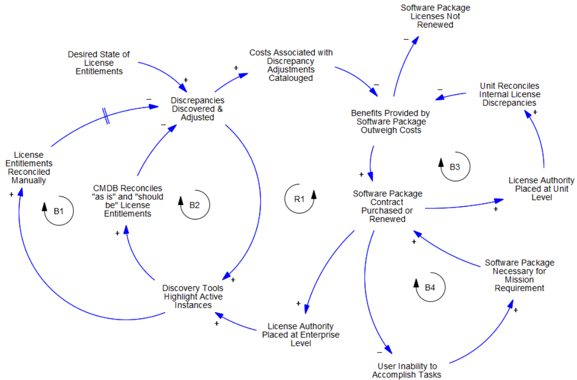
Figure 10. Enterprise License Management Systems Model.
