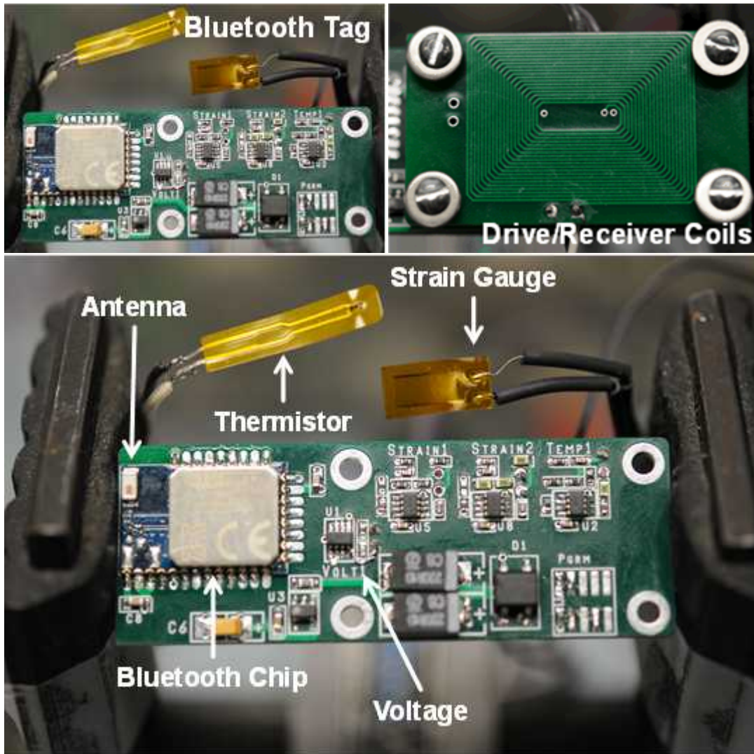
Figure 4c – Prototypical passive wireless sensor capable of simultaneously monitoring several voltages, current, strain and temperature, ideally suited for monitoring energy conversion and storage devices, including but not limited to photovoltaics, thermoelectric generators, primary and secondary electrochemical batteries, capacitors, flywheels, and various types of generators.
