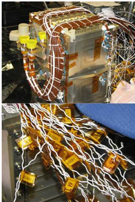
Figure 3 –2.5 kWh Li-Ion battery pack for NASA’s Mars Science Laboratory requires extensive wiring harness; more sensors are needed in such systems without the proliferation of wiring harnesses. Elimination of the wiring harness promise to increase reliability, decrease weight, and increase mass-specific power and energy.
