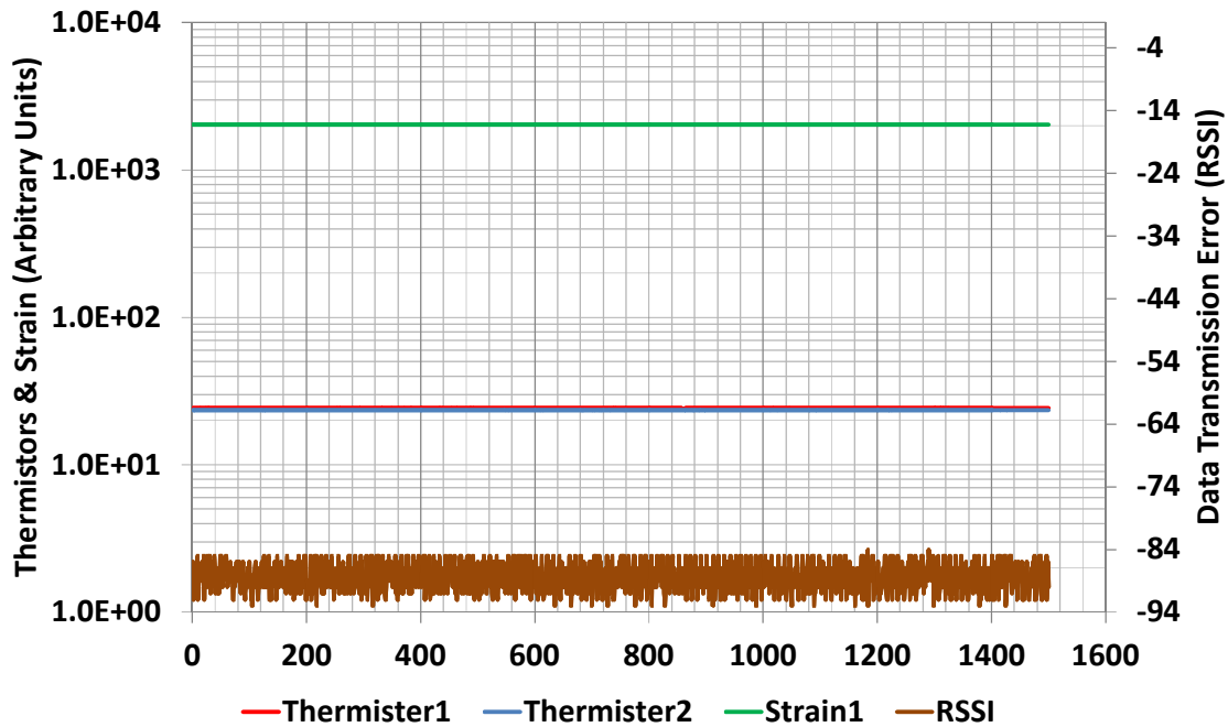
Figure 24 – Successful data transmission inside “grid storage like” electromagnetic environment, during charge and discharge of twenty 22-kV 22-kJ capacitors, from inside steel cabinet containing bank of capacitors. The two thermistors tracked ambient temperature, while the strain gauge continued to function. While a fiber optic strain gauge has been glued to the capacitor surface, the team has not yet permanently attached the wireless strain gauge to the capacitor, though this is planned. During charging, there is a slight observable contraction in the oil-filled capacitor.
