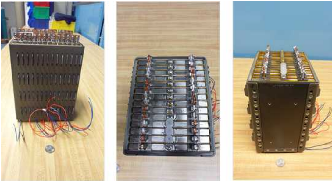
Figure 4b – These photographs shows the Yardney Technical Products 7S2P battery simulator assembled and ready for the initial testing of the Lawrence Livermore National Laboratory wireless tags and sensors.
