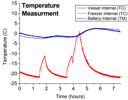
Figure 20 – This figure shows data collected from the polymer-gel lithium-ion cell with both imbedded (internal) and external temperature sensors. In this case, the cell is being discharged at a rate of approximately C/10 and controlled external temperature of approximately 0^\circ\text{C} . The internal temperature probe responds to the combined influence of Ohmic heating and external temperature cycling, as expected.
