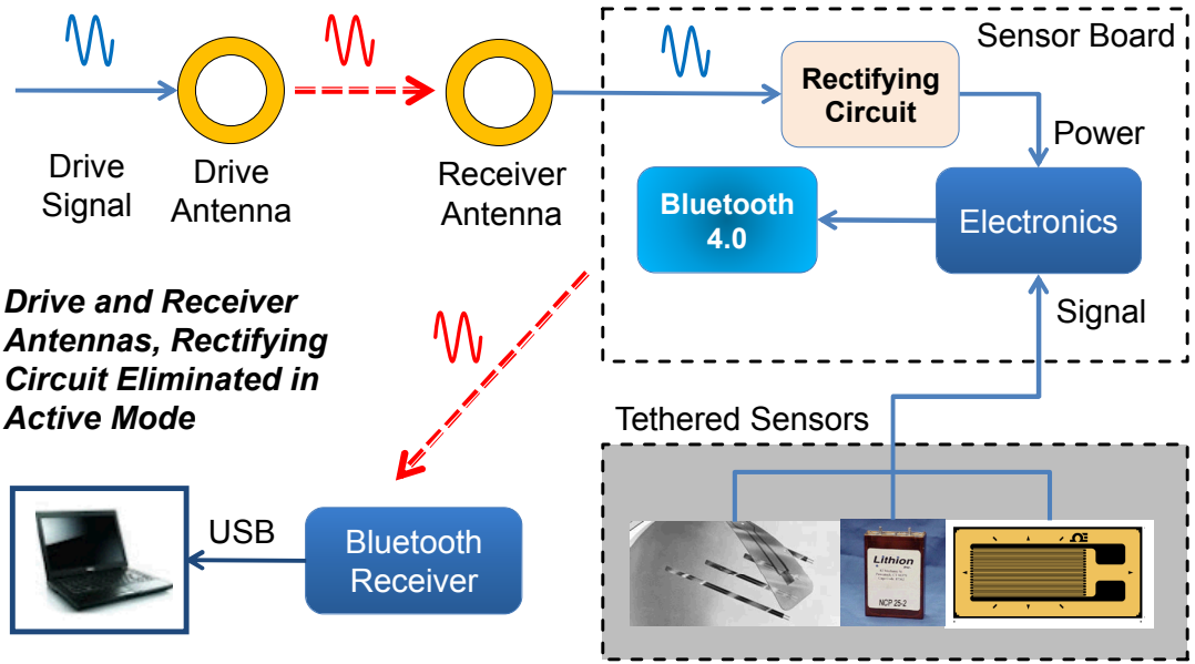
Figure 4a – The proposed wireless sensors and controllers provide a means of eliminating the massive wiring harnesses, and are capable of increasing safety, reliability, specific power, and specific energy.
