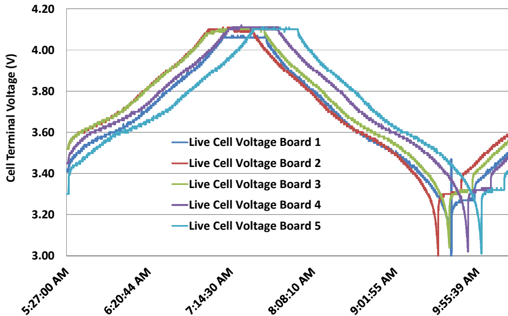
Figure 11 – Passive RFID voltage sensors following terminal voltage of individual lithium-ion cells in battery pack during charge-discharge cycling.
