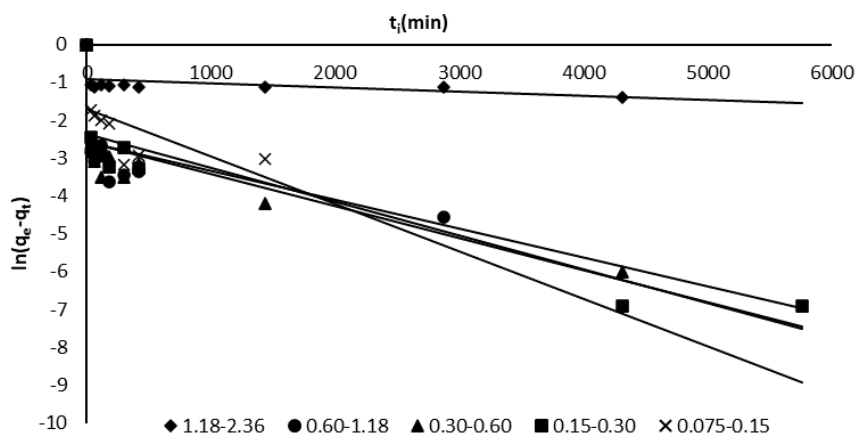
Figure 6. Linear line of plotting for PFO with different particle sizes.
