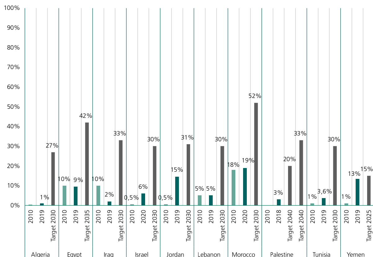
Overview of Renewable Shares in Electricity Generation 2010 and 2019/20 and Renewable Targets
