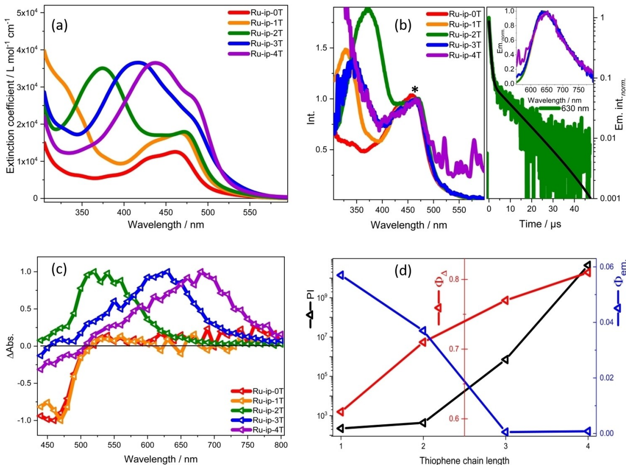
Figure 2. (a) Absorption spectra for the Ru-ip- n T complexes in water. (b) Excitation spectra of the Ru-ip- n T complexes in water at 640 nm emission normalized to the MLCT band at 480 nm (*, left); bi-exponential emission decay of Ru-ip-2T with lifetimes of 0.6 μs and 11 μs at 630 nm (right); Inset: Emission spectra of Ru-ip- n T complexes normalized to their respective maxima. (c) Nanosecond TA spectra of Ru-ip- n T complexes in aerated water normalized to their respective maxima at λ ex : 410 nm at 300 ns. (d) Relationship between the PI values (black y-axis), singlet-oxygen quantum yield Φ Δ (red y-axis) in aerated MeCN (excitation at 450 nm) and fluorescence quantum yield Φ em. (blue y-axis) in deaerated water (excitation at 450 nm) with increasing thiophene chain length (x-axis). (1) The PI is defined as the ratio of EC 50 dark to EC 50 visible light values in SK-MEL-28 cells.
