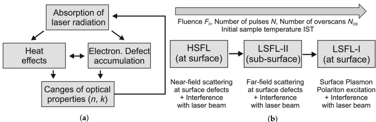
Figure 11. a) Scheme of iterative intra-pulse effects changing the optical properties of a dielectric (polycarbonate) during laser irradiation. b) Scheme of the evolution/transition between different types of LIPSS at the surface of dielectrics. Reproduced under the terms of a Creative Commons BY 4.0 license. [90] Copyright 2019, The Authors, published by MDPI.
