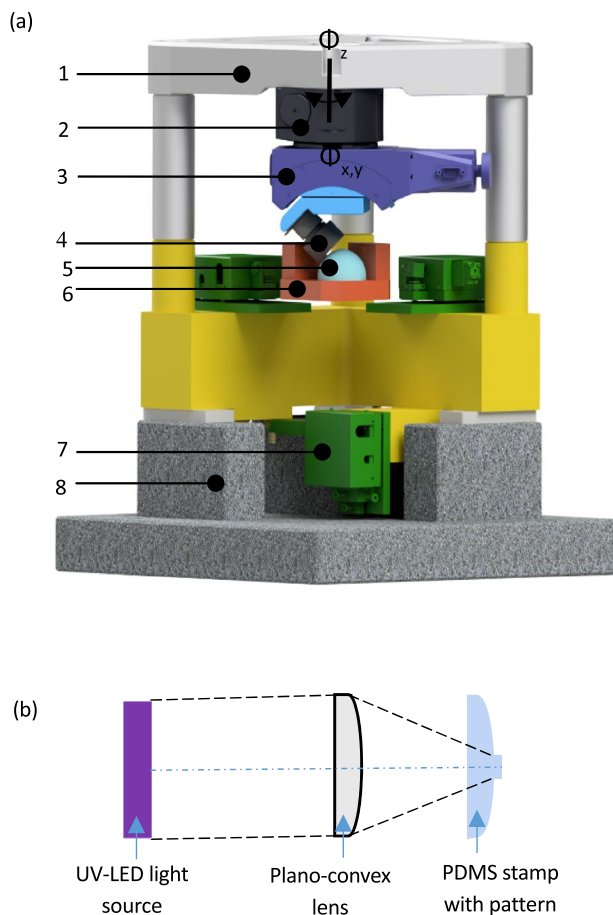
Fig. 1 a Basic model of nanopositioning and nanomeasuring machine with additional rotating nanoimprint tool: 1 metrological frame of NMM-1; 2 rotation stage ( \phi_z ); 3 goniometer stage ( \phi_{x,y} ); 4 NIL tool; 5 substrate; 6 mirror corner of NMM-1 (moved in x, y, z ); 7 interferometer of NMM-1; 8 metrological frame of NMM-1. b Detailed schematic of developed NIL tool
