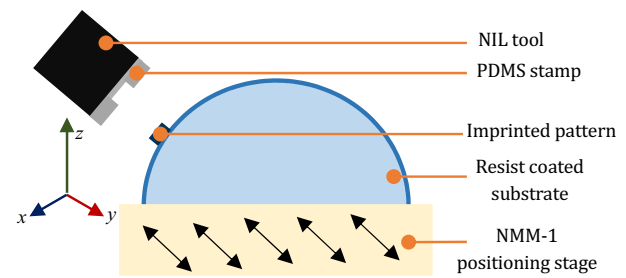
Fig. 2 Orthogonal molding and demolding on edges of curved surface enabled by the diagonal movement (shown by arrows) of the positioning stage
