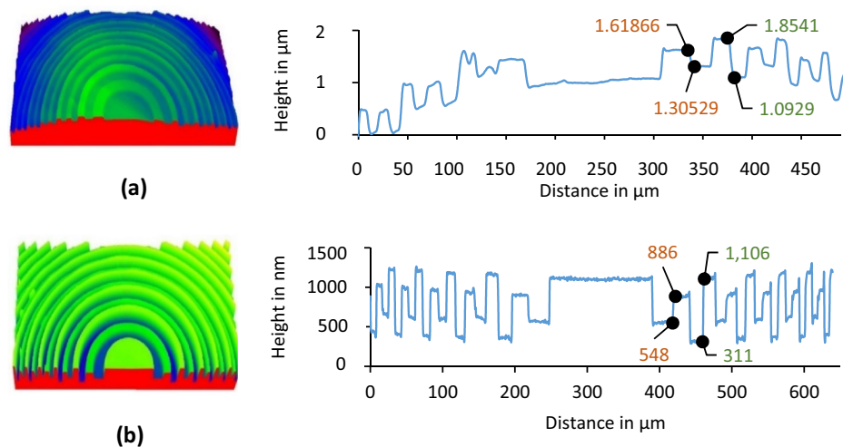
Fig. 4 3-D laser scanning microscope images and corresponding structure profiles of (a) imprinted pattern using rotating NIL tool on the edge of the plano-convex lens (measured using a profilometer); b master pattern on PDMS stamp
