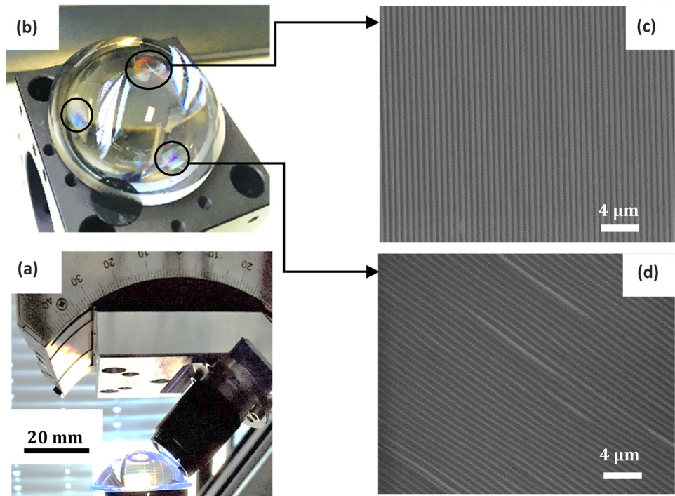
Fig. 3 a Soft UV-NIL process at the edge of the plano-convex lens; b imprinted plano-convex lens at angles of c 90^\circ ( top ) and d 45^\circ ( edge ) of the rotating NIL tool
