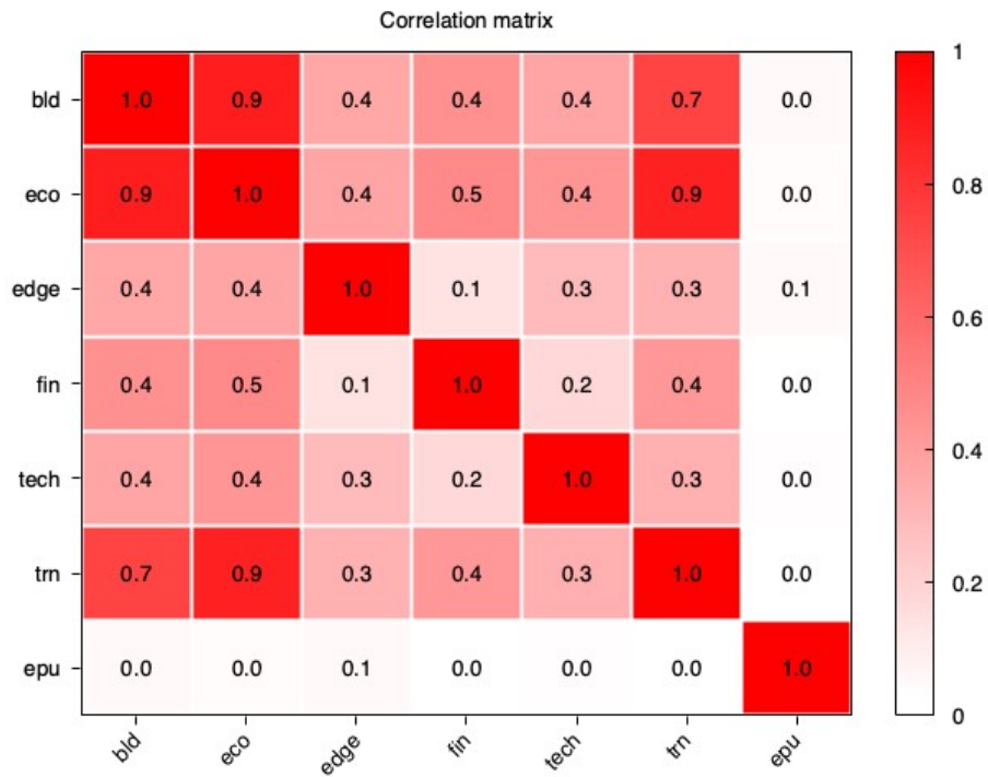
Figure 3: Correlation matrix
