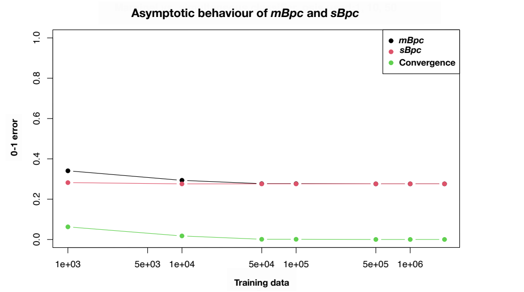
Figure 1. The classification error of the marginal and simultaneous classifiers with datasets from PD distribution with \psi \in (1, 10, 50) , as well as the convergence of their labellings. Rows 2 and 3 in Table 1 are included in the figure.
