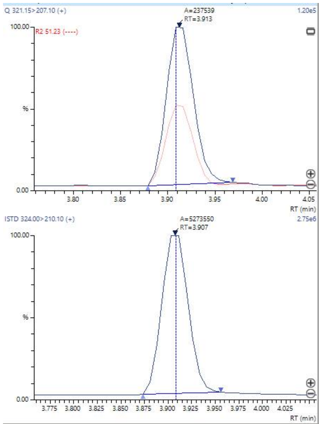
Figure 2. (A) LC-MS/MS plot of mycophenolic acid in the urine sample of Patient 1 above and the internal standard below. The graph shows a tracing in blue which is the quantifier ion (mass = 207.1) and a tracing in red which is the qualifier ion at mass = 159.1. The peak below with only a single blue tracing is the tracing of the deuterium-labeled mycophenolic internal standard (mass = 210.1). The mycophenolic acid internal standard has a virtually identical retention time to mycophenolic acid in the patient, but the quantifier ion is mass = 210.1 because of three deuterium atoms in the internal standard; (B) LC-MS/MS plot of mycophenolic acid in the urine sample of Patient 2. The upper graph of the patient shows a tracing in blue which is the quantifier ion (mass = 207.1) and a tracing in red which is the qualifier ion at mass = 159.1. The peak below with only a single blue tracing is the tracing of the deuterium-labeled mycophenolic internal standard (mass = 210.1).
