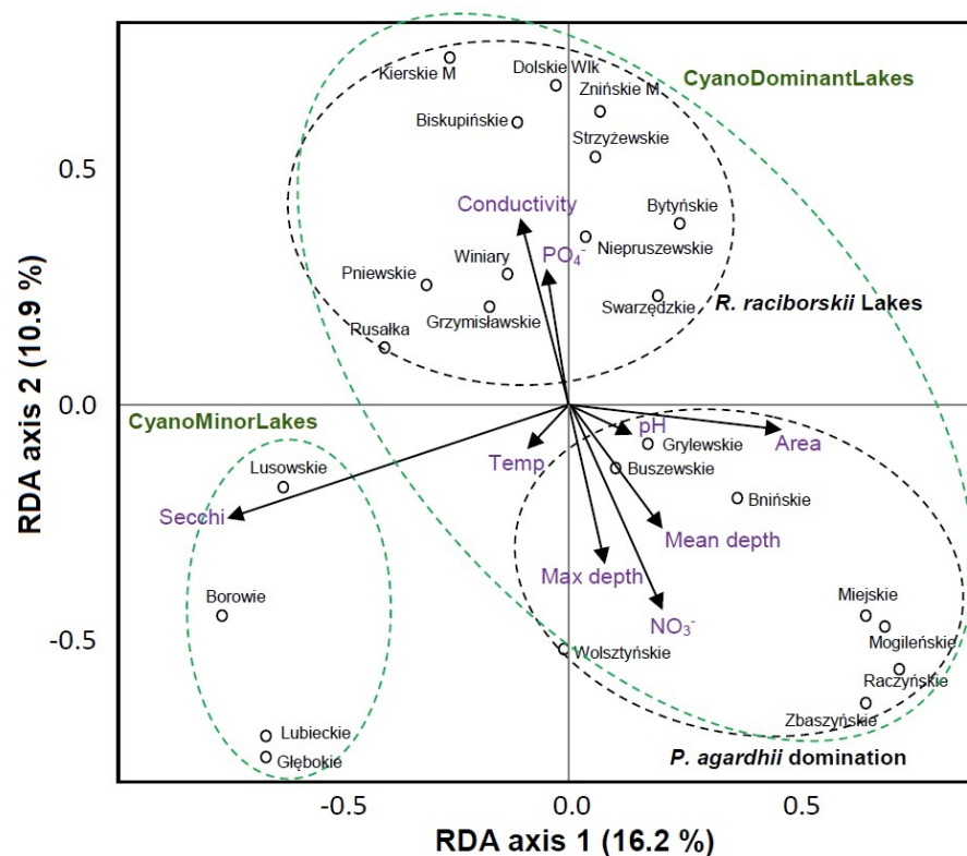
Figure 3. Redundancy analysis plot for phytoplankton in the studied lakes divided into two main groups. The variation explained by each axis has been plotted on the x-axis (RDA 1—eigenvalue 0.103) and y-axis (RDA2—eigenvalue 0.070).
