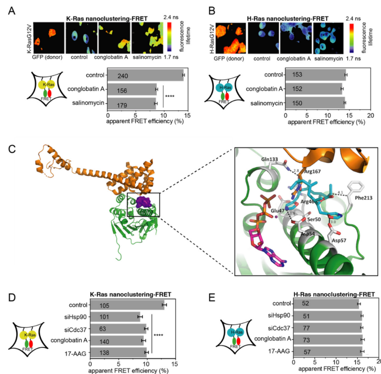
Figure 1. Conglobatin A selectively targets K-Ras via the inhibition of Hsp90/Cdc37. (A,B) FLIM-FRET images of HEK cells transfected with FRET-pairs of mGFP-/mCherry-K-RasG12V ( A , top) or mGFP-/mCherry-H-RasG12V ( B , top). The labelling indicates donor-only control or treatments. A decrease in the fluorescence lifetime indicates an increase in FRET due to nanoclustering. The transfected cells were treated with 0.1% DMSO vehicle control, 2 \mu M conglobatin A, or 1.3 \mu M salinomycin for 24 h. The nanoclustering-FRET analysis by treatment for K-RasG12V ( A , bottom) or H-RasG12V ( B , bottom). The numbers in the bars indicate the number of analyzed cells; n = 3 independent biological repeats. (C) Conglobatin A (purple surface) was docked into the crystal structure of human N-Hsp90 (green; PDB ID 3T0Z). The docked complex was overlaid on top of the crystal structure of yeast N-Hsp90 in a complex with human Cdc37 (PDB ID 1US7), of which only Cdc37 is depicted (orange). The magnification shows the details of how conglobatin A (cyan sticks) sterically blocks and disturbs critical interactions, notably between Glu47 of Hsp90 (gray sticks) and Arg167 of Cdc37 (orange sticks) at the interface of the complex. ATP is shown as magenta sticks, and magnesium is shown as a deep purple sphere. The polar interactions between conglobatin A and Hsp90 are shown as dashed lines, with distances in Ångströms. (D,E) The K-RasG12V- ( D ) and H-RasG12V- ( E ) nanoclustering-FRET in HEK cells co-transfected with mGFP- and mCherry-tagged RasG12V, together with 50 nM siRNA Hsp90, siRNA Cdc37, or 50 nM scrambled siRNA for compound/vehicle (control) treated samples. The next day, the cells were treated for 24 h with 0.1% DMSO vehicle control, 2 \mu M conglobatin A, or 2 \mu M 17-AAG. The numbers in the bars indicate the number of analyzed cells. The number of independent biological repeats n = 3 for K-Ras and n = 1 for H-Ras. **** p < 0.0001 .
