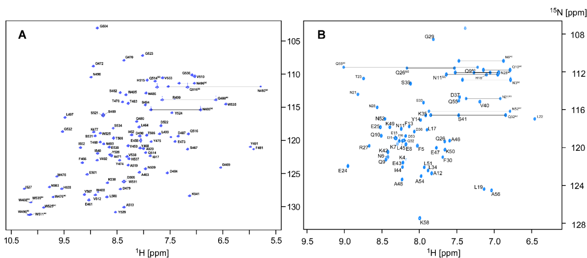
Figure 1. (A) Two-dimensional [\text{}^1\text{H}, \text{}^{15}\text{N}] -HSQC spectrum of [20\% \text{}^{13}\text{C}, 100\% \text{}^{15}\text{N}] -labeled CBM64 recorded at the ^1\text{H} frequency of 850 MHz, 303 K with the assignment using one letter amino-acid codes (residues 458–541). (B) Two-dimensional [\text{}^1\text{H}, \text{}^{15}\text{N}] -HSQC spectrum of [20\% \text{}^{13}\text{C}, 100\% \text{}^{15}\text{N}] -labeled SpaC with the assignment using one letter amino-acid codes (residues 4–58). The sidechains are marked by “sc”. Identified sidechain amides of glutamine ( \text{Q}^{\text{sc}} ) and asparagine ( \text{N}^{\text{sc}} ) are indicated by horizontal lines.
