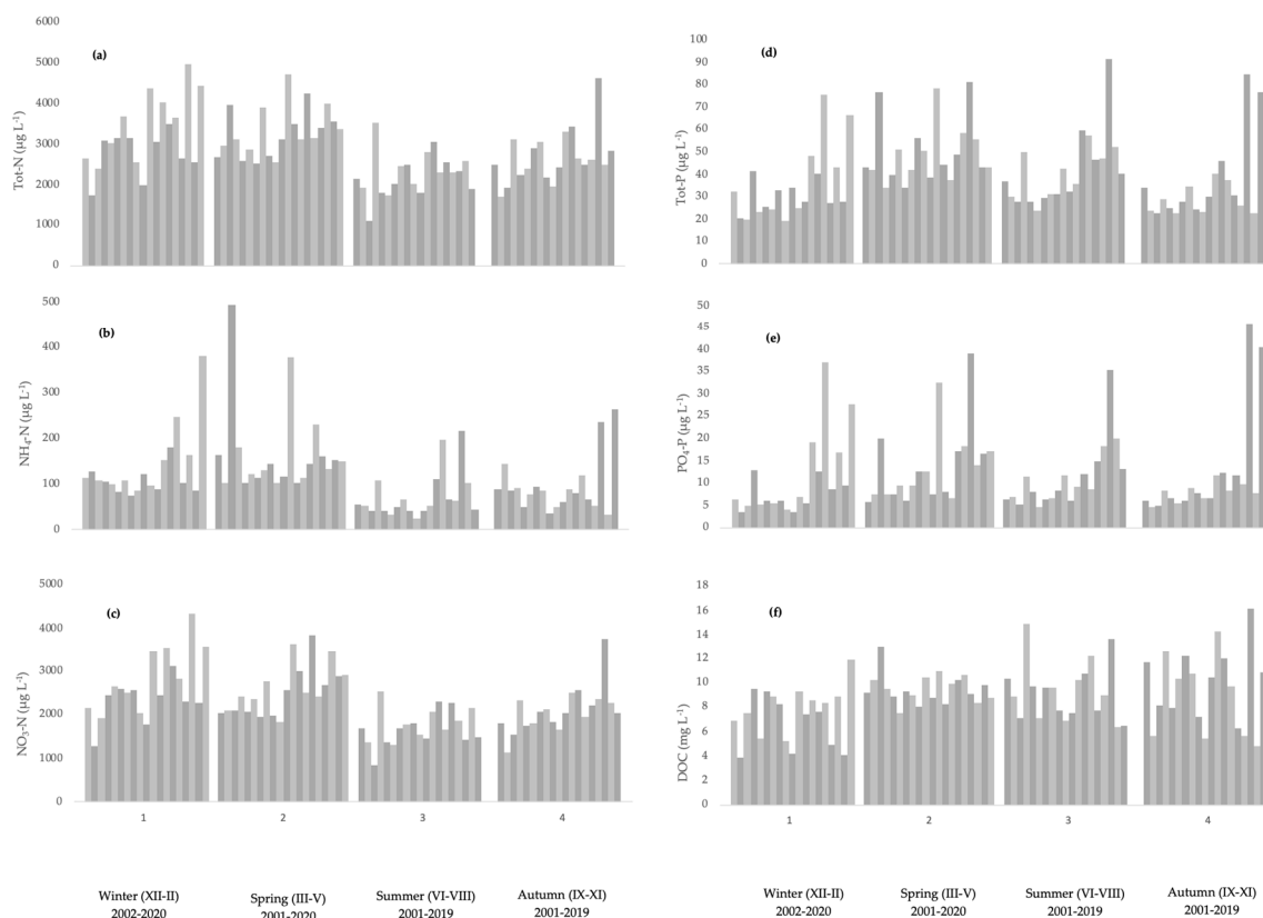
Figure 3. Average seasonal (a) Tot-N-, (b) \text{NH}_4\text{-N} -, (c) \text{NO}_3\text{-N} -, (d) Tot-P-, (e) \text{PO}_4\text{-P} -, (f) DOC-concentrations in the Koiransuolenoja stream between 2001 and 2020 (even years with light gray, odd years with dark gray). XII–II = December–February, III–V = March–May, VI–VIII = June–August, IX–XI = September–November.
