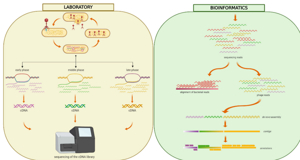
Figure 1. Workflow of the RNA-seq approach. Freshly diluted Y. ruckeri RS41 bacteria were grown until OD_{600} = 0.6 and then infected with phage YerA41 at MOI equal to 10 or 50. The culture was washed with LB to remove the unbound phage particles, and thus prevent re-infection of bacterial cells at later stages of the experiment. Samples for RNA isolation were taken at different time points p.i. (0, 5, 15, 33, 45, 63, 75, 92 min). After the removal of bacterial rRNA, the prepared libraries were sequenced. The obtained sequencing reads were quality filtered and aligned against Y. ruckeri PBH2 chromosome (Acc.no. LN681231.1) and plasmids pYR2 (Acc.no. LN681229.1) and pYR3 (Acc.no. LN681230.1). The reads that failed to align to these reference sequences were merged together and assembled using Velvet [13] and SPAdes [14]. The obtained assembled sequences were blasted against the NCBI nucleotide collection and contigs showing high identity rates with Yersinia strains were excluded. The phage genomic scaffolds were auto-annotated using Rapid Annotation Using Subsystem Technology (RAST) [20]. Presence of suitable ribosomal binding sites in front of each predicted start codon was confirmed. Figure was created using BioRender ( https://app.biorender.com ).
