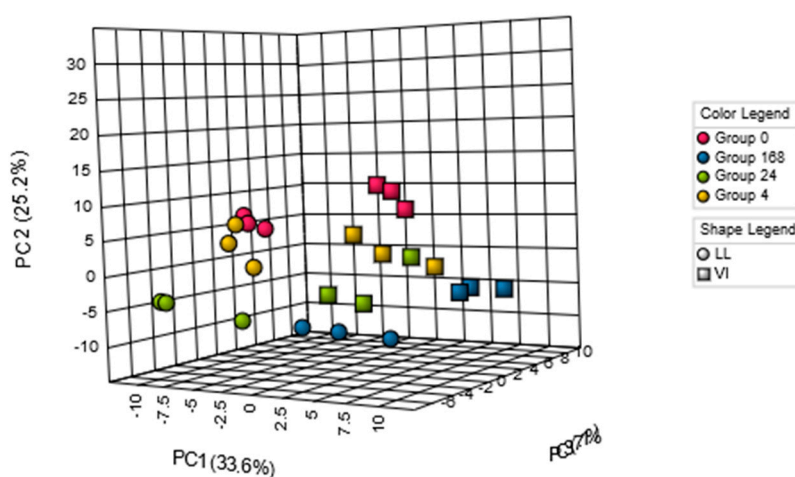
Figure 1. Classification of pig LL and VI muscle samples of different postmortem aging period by PCA. Pig LL and VI muscles were aged during 0, 4, 24, 168 h postmortem.
