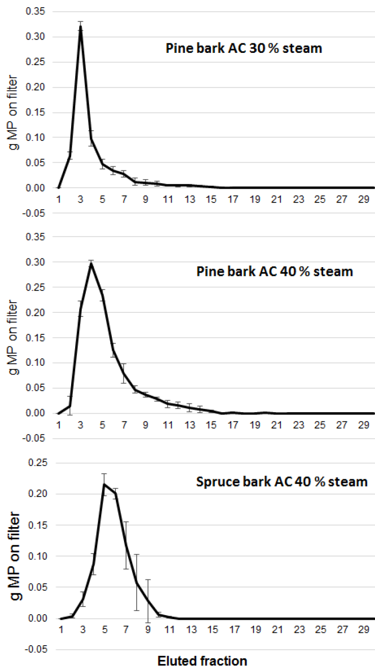
Figure 6. Retention of 10 µm microplastics particles on activated biochar.
