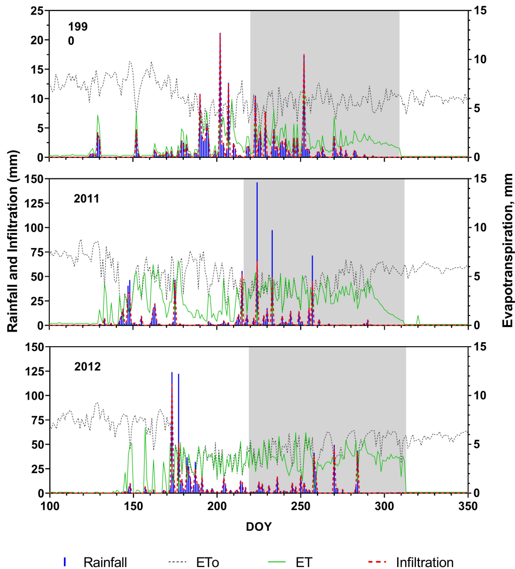
Figure 1. Daily rainfall (CFRS) and AquaCrop -simulated Penman-Montieth reference evapotranspiration (ET 0 ), evapotranspiration (ET), and infiltration for day of the year (DOY) 100 to 350 in 1990, 2011, and 2012. Shaded area covers the growing season. Note the different y-axis scales used for 1990 rainfall and infiltration compared to 2011 and 2012. ET and infiltration values are for the no biochar scenario (BC0) (simulated biochar amendments had little effect on ET and infiltration).
