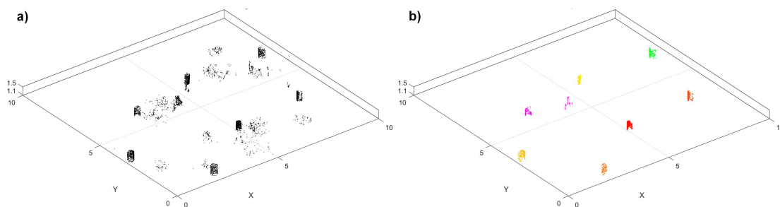
Figure 2. A 10 m × 10 m sub-sample of an original sample plot to illustrate the stage-one tree detection. First, a horizontal point cloud slice was delineated from the normalized point cloud (a). Then, points were segmented into clusters, and vertical and cylindrical point cloud structures were considered to represent cross-sections of trees (b).
