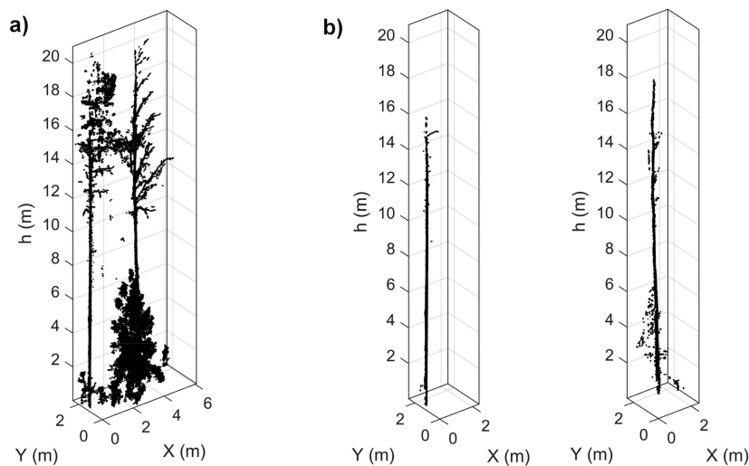
Figure 4. An example of the stage-two tree detection. Multiple trees in a tree-wise point cloud (a) were detected using point cloud filtering and clustering. Stem points were extracted separately for both trees (b).
