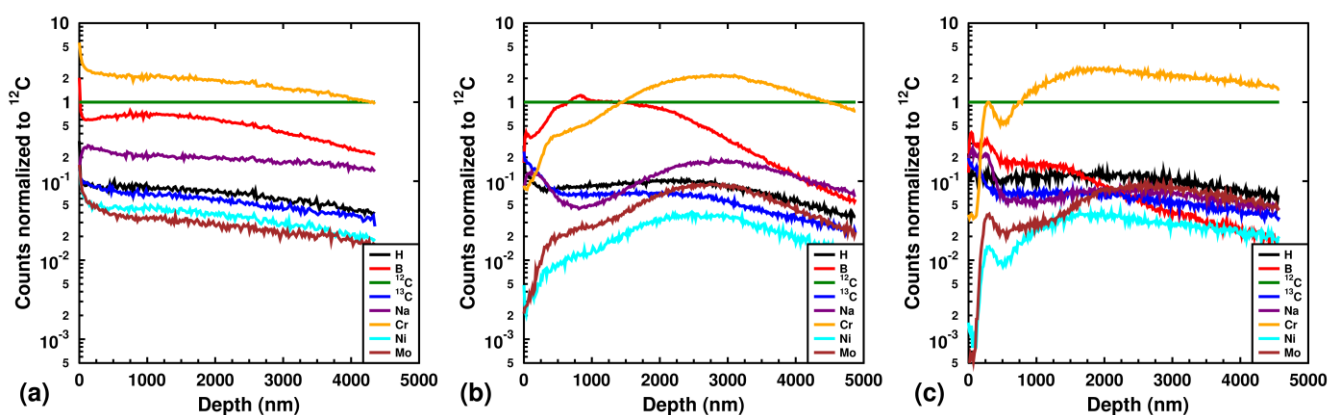
Figure 6: SIMS depth profile of impurities measured from (a) HM58TM100vTE9P3T2, (b) HM58TM300hTE8P8T2 and (c) HM58TM200hTE4P8T1. In (a) most of the impurities show their maxima on the surface excluding boron which has its peak at around the depth of 1 \mu\text{m} . In (b) and (c) there are several maxima for many impurities suggesting complex impurity layers in the deposition areas.
