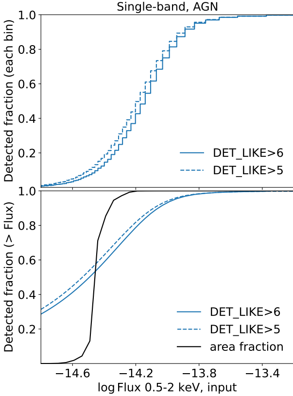
Fig. 10. Simulation-measured completeness of AGN in the single-band detected catalogue as a function of the 0.5–2 keV input flux ( \text{erg cm}^2 \text{s}^{-1} ) in differential ( upper panel ) and cumulative manners. The solid and dashed blue lines indicate the detected AGN with \text{DET\_LIKE} > 6 and \text{DET\_LIKE} > 5 , respectively. For comparison, we also plot the sky coverage area curve measured by ersensmap adopting \text{DET\_LIKE} \geq 5 normalised to a total area of 1 (black line).
