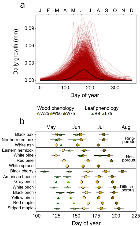
Figure 3. Wood and leaf phenology over 1999–2003 across individuals (red curves) and averaged per species (colored symbols). Error bars indicate 95% credible intervals (stem phenology) or standard deviation (leaf phenology). W25: 25% of annual diameter growth; W50: 50% of annual diameter growth; W75: 75% of annual diameter growth; BB: bud break; L75: leaf out. (a) Daily modeled growth of all 1992 tree-years. The black lines indicate 10th, 50th and 90th quantiles of daily growth rates. (b) Posterior mean estimates of wood phenology per species. Average leaf phenology measured at the site for corresponding species and years is also presented when available.
