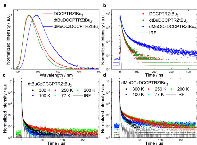
Figure 4. Photoluminescence of emitters in PVK film (10 wt%). (a) Steady-state PL spectra ( \lambda_{\text{exc}} = 345 nm), (b) prompt PL decay of all emitters, (c) delayed PL decay component at different temperatures of dtBuCzDCCPTRZtBu 2 and (d) dMeOCzDCCPTRZtBu 2 . For transient PL ( \lambda_{\text{exc}} = 378 nm).
