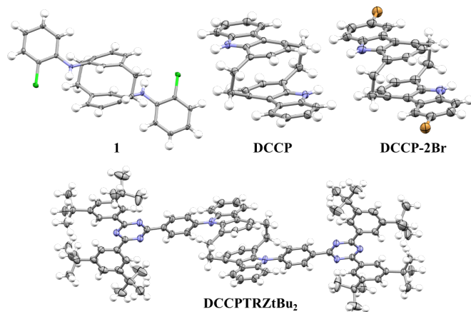
Figure 2. Thermal ellipsoid plots of the crystal structure of 1 , DCCP , DCCP-2Br , and DCCPTRz2Bu 2 . Ellipsoids are plotted at the 50% probability level.
