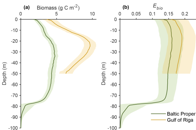
Figure 5. Depth distribution of benthic fauna biomass and the bioturbation coefficient E_{\text{bio}} in the upper 100 m of the Baltic Proper and Gulf of Riga. Averages (lines) and standard deviations (shaded areas) of biweekly values (2000–2020) in the default model run ( E_{\text{max}} = 0.3 ).
