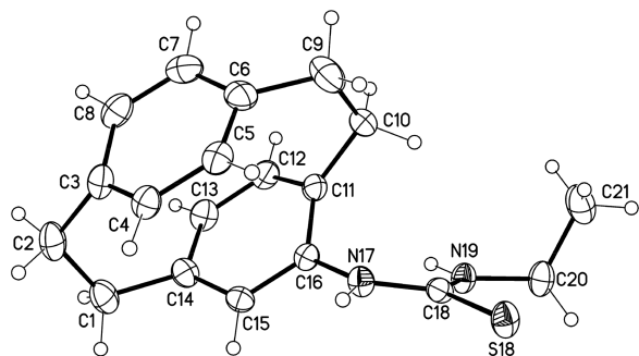
Figure 4. Molecular structure of one of the crystallographic independent molecules of compound 11d (displacement parameters are drawn at the 50% probability level).
