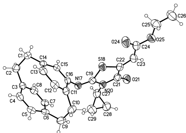
Figure 6. Molecular structure of compound 14e (displacement parameters are drawn at 50% probability level).
