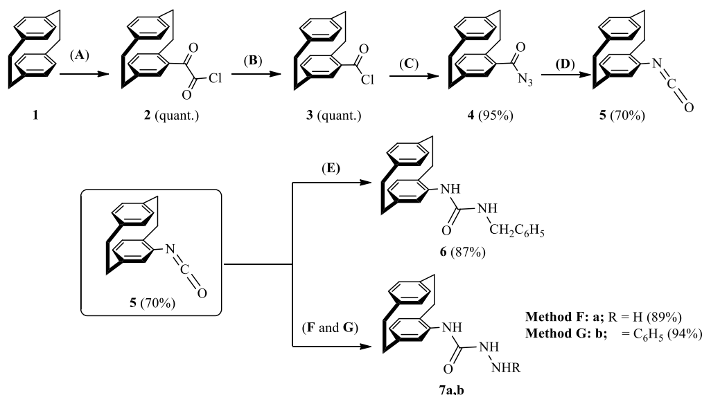
Scheme 1. Synthesis of 1 N -Benzyl-3- N -[2.2]paracyclophanylurea ( 6 ) and N -(4'-[2.2]Paracyclophanyl)hydrazinecarboxamides 7a and 7b a
