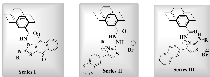
Figure 1. Different series of paracyclophanyl-thiazole derivatives (I–III) as anticancer agents.
