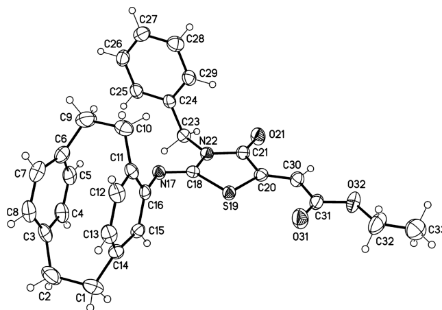
Figure 5. Molecular structure of compound 14b (minor disordered parts omitted for clarity, displacement parameters are drawn at 50% probability level).
