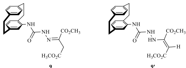
Figure 2. Additive products 9 and 9' from the reaction between 7a and 8a .
