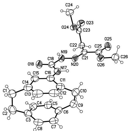
Figure 3. Molecular structure of compound 9 (displacement parameters are drawn at the 50% probability level).
