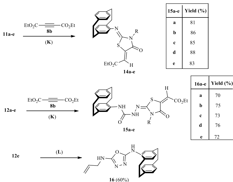
Scheme 4. Synthesis of Thiazoles 14a – 14e and 15a – 15e in Addition to 1,3,4-Oxadiazole Derivative 16 a
