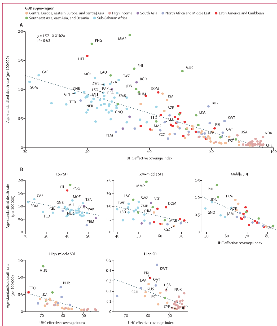
Figure 3: Scatterplot of age-standardised diabetes death rate at ages younger than 25 years by UHC index in 2019 globally (A) and by SDI quintile (B). The diagonal line is the death rate at each UHC index as estimated by linear regression. Country super-regions are indicated by colours. UHC=universal health coverage.
