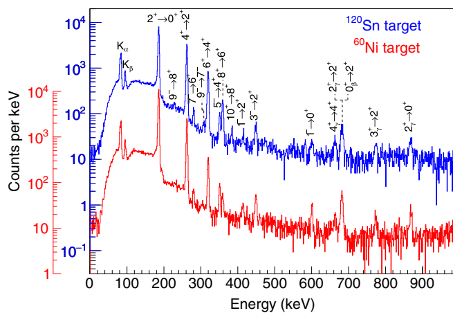
FIG. 5. Spectra of \gamma rays emitted following Coulomb excitation of ^{222}\text{Rn} using a ^{120}\text{Sn} target (blue) and a ^{60}\text{Ni} target (red) observed in coincidence with recoiling target nuclei. The \gamma -ray energies were corrected for Doppler shift assuming they are emitted from the scattered projectile. Time-random coincidences between Miniball and CD detector have been subtracted. The spectra were obtained by sorting the data in the segment mode.
