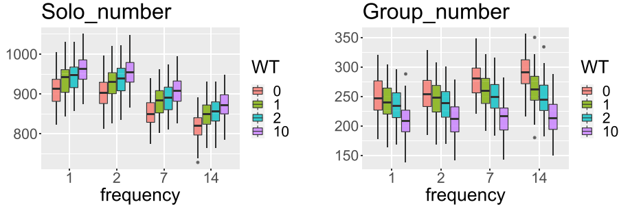
Fig. 11. The Solo and Group results with 0,1,2,10 weight on the waiting time.
