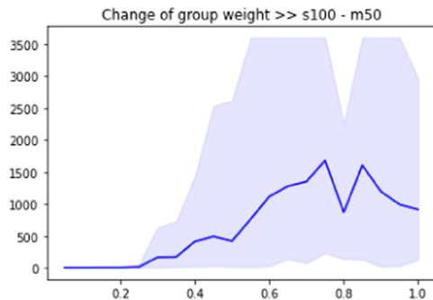
Fig. 5. Increasing the group weight, with 100 students and 50 mentors.
