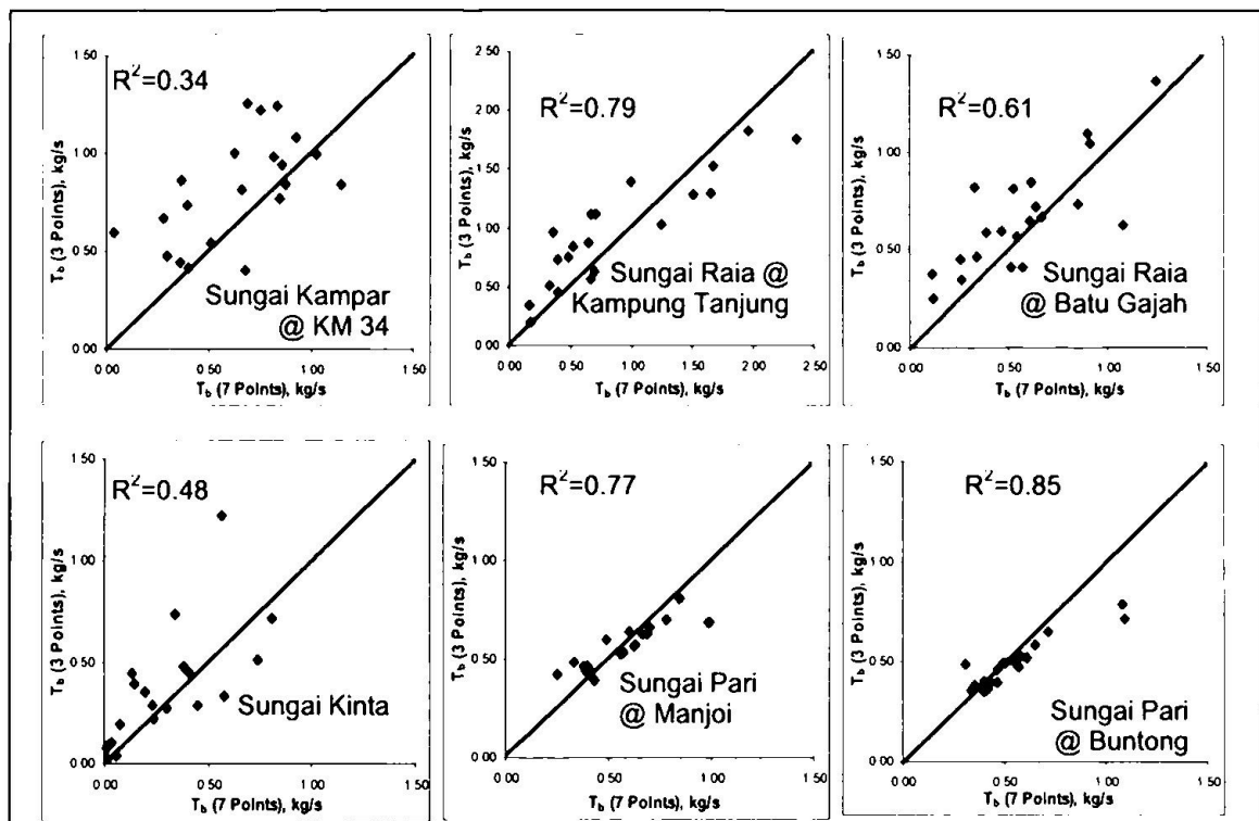
Figure 2.5: Comparison of Computed Bed Load Transport Rate between Seven-Point Measurement Method and Three-Point Measurement Method (Ab. Ghani et al., 2003)
