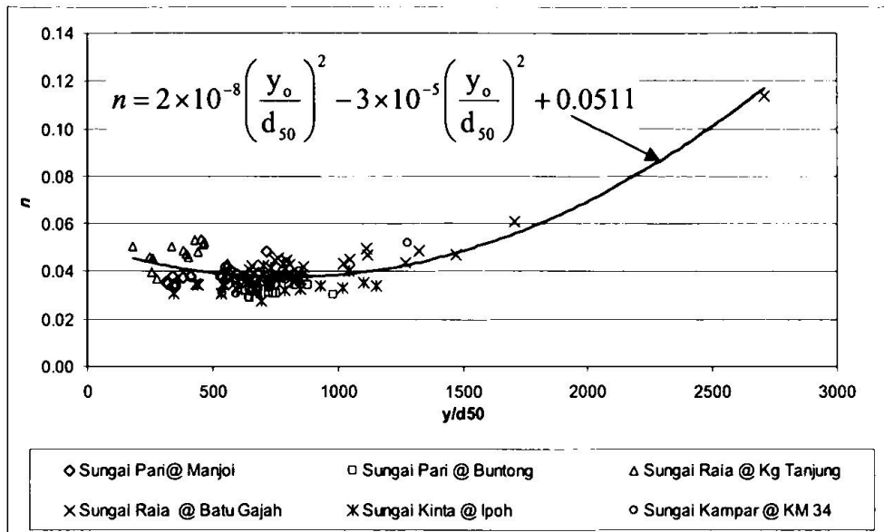
Figure 2.7: Development of Equation 2.7 to determine the Value of n based on y/d_{50} (Abdul Ghaffar, 2003)
