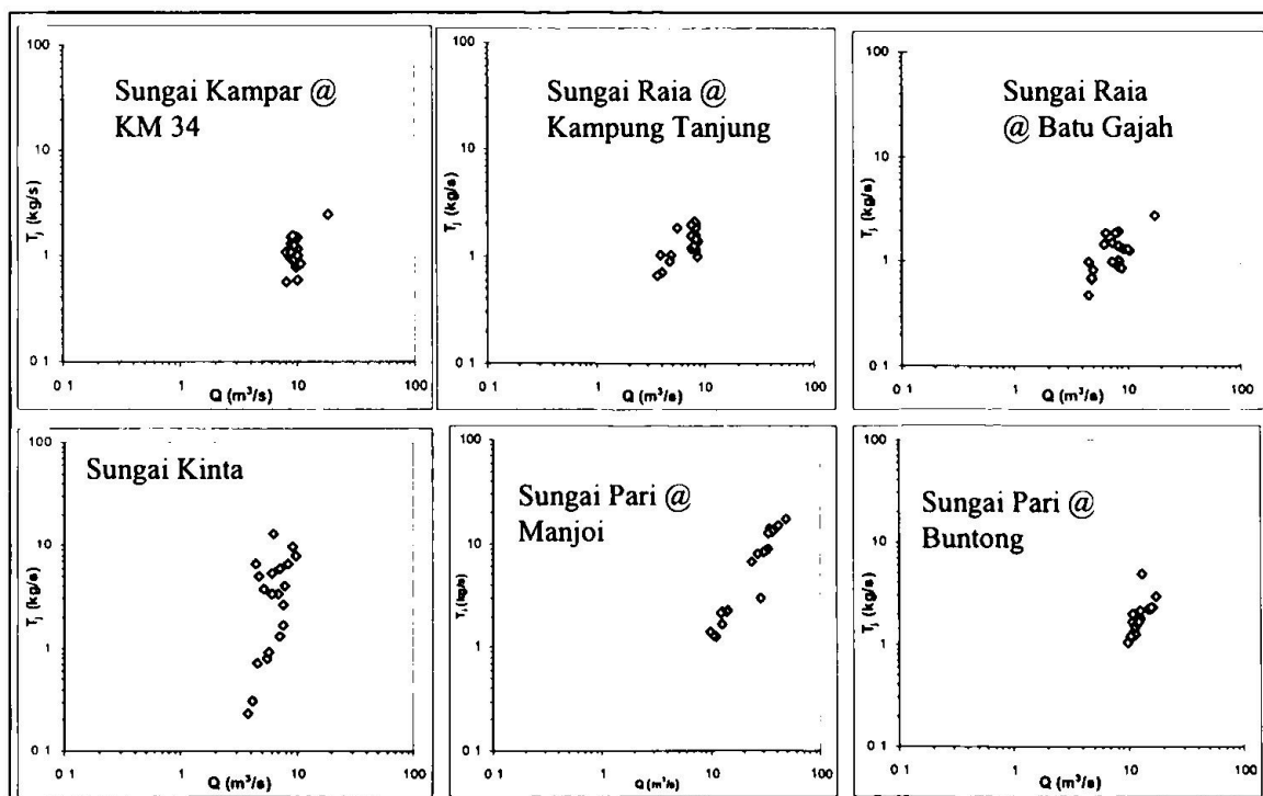
Figure 2.4: Total Load Rating Curve for Sungai Kinta Catchment (Ab. Ghani et al., 2003)
