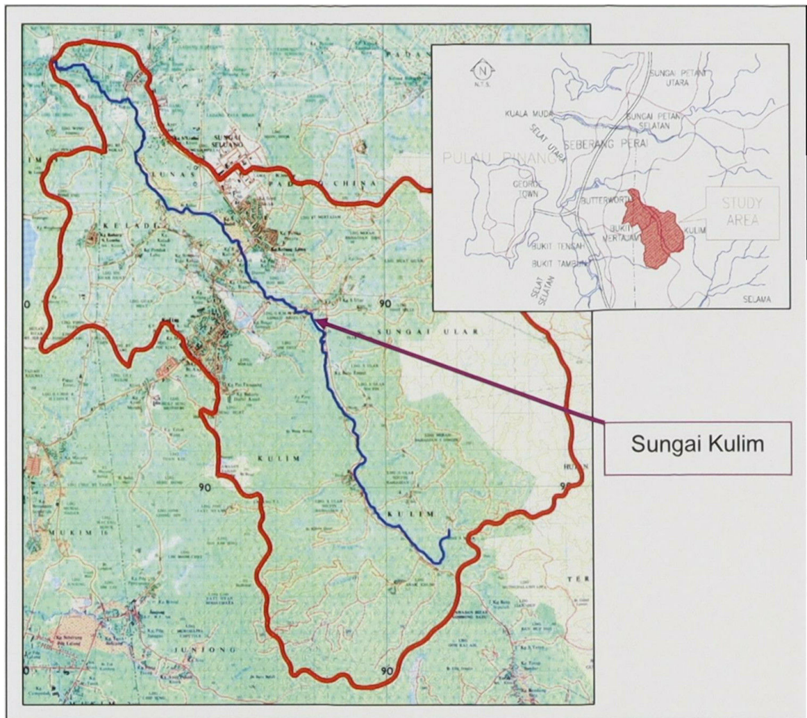
Figure 1.1: Topographical Map of Sungai Kulim Catchment
