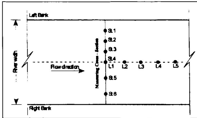
Figure 2.14: Layout of Measurement Stations and Locations (Abdel-Fattah et al., 2004)
