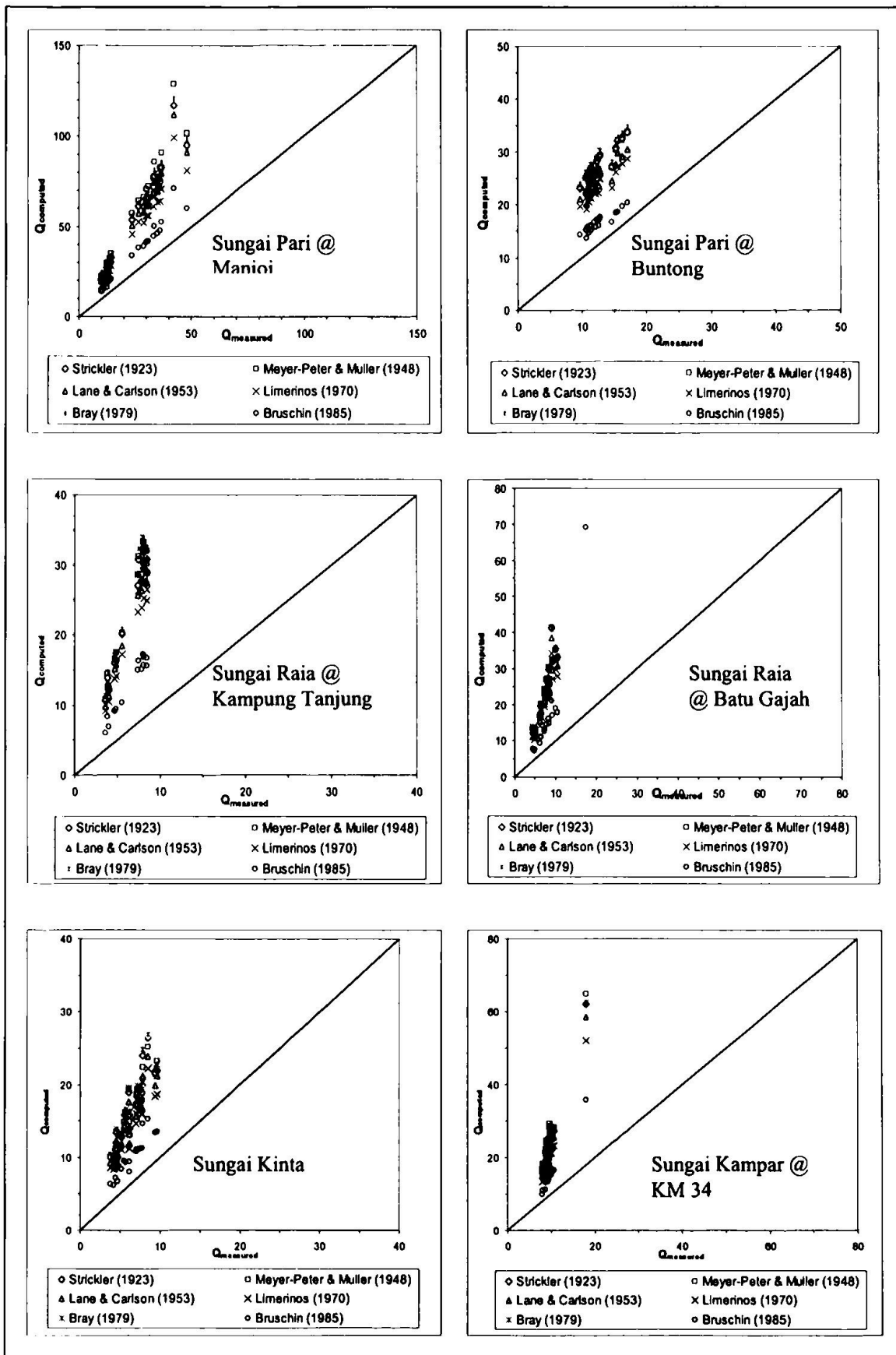
Figure 2.6: Evaluation of Manning's Equations using Equations 2.1 to 2.6 (Abdul Ghaffar, 2003)
