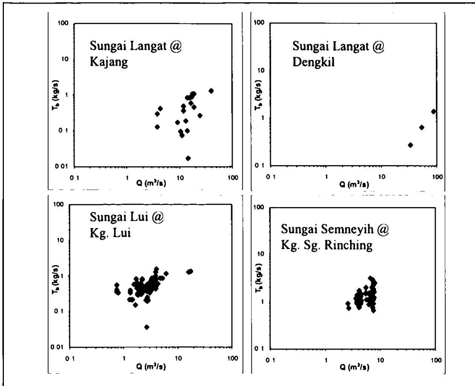
Figure 2.10: Bed Load Rating Curves for Sungai Langat Catchment (Ariffin, 2004)
