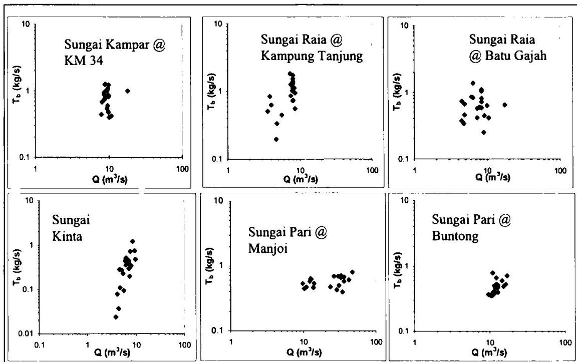
Figure 2.3: Bed Load Rating Curves for Sungai Kinta Catchment (Ab. Ghani et al., 2003)
