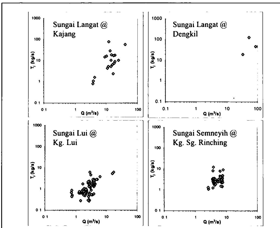
Figure 2.11: Total Load Rating Curves for Sungai Langat Catchment (Ariffin, 2004)
