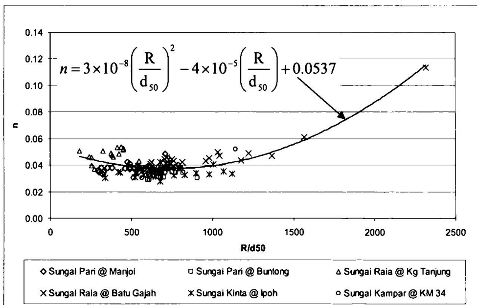
Figure 2.8: Development of Equation 2.8 to determine the value of n based on R/d_{50} (Abdul Ghaffar, 2003)
