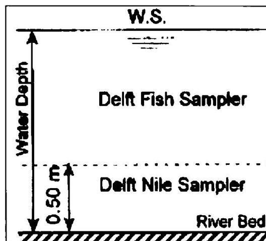
Figure 2.13: Sketch of Measuring Technique (Abdel-Fattah et al., 2004)
