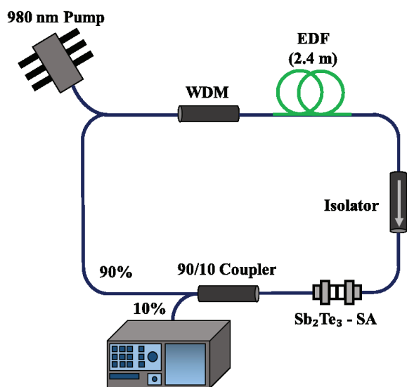
Fig. 2. Configuration setup of the Q-switched EDFL.
