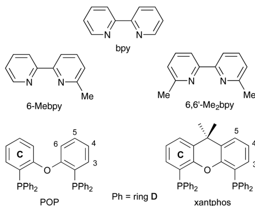
Scheme 1 Structures of 2,2'-bipyridine, 6-methyl-2,2'-bipyridine, 6,6'-dimethyl-2,2'-bipyridine, and of the P ∧ P ligands with numbering for spectroscopic assignments.
