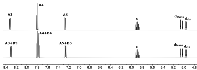
Fig. 1 Part of the 500 MHz ^1\text{H} NMR spectra of ligands 1 (top) and 2 (bottom) in acetone- d_6 . Chemical shifts in \delta/\text{ppm} . See Fig. S3 and S8 \ddagger for the complete spectra. Atom labels are defined in Scheme 2.
