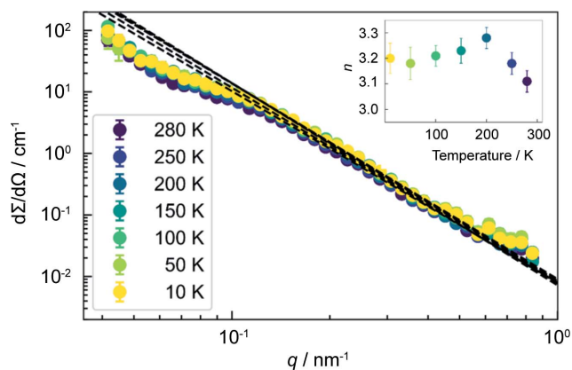
Figure 8 The temperature dependence of the azimuthally averaged (over \pm 10^\circ ) 1D total (nuclear + magnetic) SANS cross section d\Sigma/d\Omega measured along the field direction ( \mathbf{q} \parallel \mathbf{H}_0 ) and at the highest applied field value of 7 T (log–log scale). Dashed lines show the extrapolation of d\Sigma/d\Omega \propto q^{-n} . The Porod fits were restricted to 0.25 \leq q \leq 0.46 \text{ nm}^{-1} . (Inset) The temperature dependence of the asymptotic power-law exponent n .
