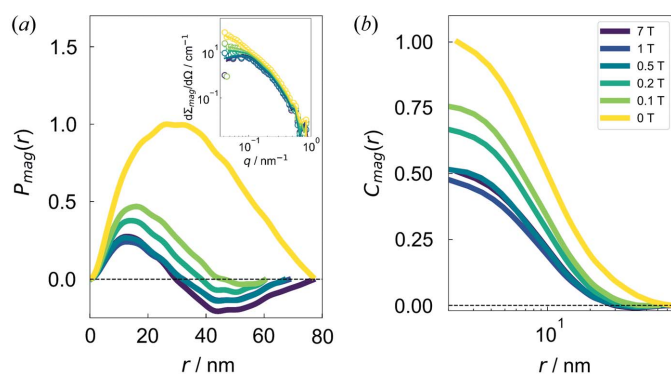
Figure 5 (a) The field dependence of the magnetic distance distribution function P_{\text{mag}}(r) at 280 K. The P_{\text{mag}}(r) values were computed numerically via an indirect Fourier transform (IFT) of the experimental d\Sigma_{\text{mag}}/d\Omega data shown in Fig. 4(b). Note that for comparison with the results obtained at lower temperatures, as summarized in Appendix C, the P_{\text{mag}} at each field has been normalized by the maximum peak intensity value obtained at remanence. (Inset) A comparison between the experimental d\Sigma_{\text{mag}}/d\Omega plotted in Fig. 4(b) (coloured open circles) and the reconstructed d\Sigma_{\text{mag}}/d\Omega based on the IFT of the numerically computed P_{\text{mag}} shown in Fig. 5(a) (coloured solid lines). (b) The corresponding magnetic correlation function C_{\text{mag}}(r) = P_{\text{mag}}(r)/r^2 (semi-logarithmic scale).
