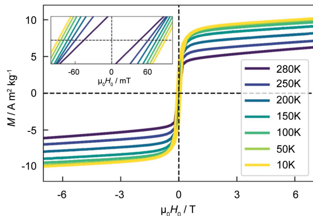
Figure 3 Magnetization curves for the \text{Ni}_{50}\text{Mn}_{45}\text{In}_5 alloy measured at the selected temperatures of 280, 250, 200, 150, 100, 50 and 10 K. (Inset) An enlargement of the magnetization curves between \pm 100 \text{ mT} .
