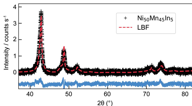
Figure 2 XRD pattern for \text{Ni}_{50}\text{Mn}_{45}\text{In}_5 alloy (Cu K\alpha radiation) (black crosses). The red dashed line shows the XRD data refinement using the Le Bail fit (LBF) method implemented in the FULLPROF software (Rodríguez-Carvajal, 1993) and considering two tetragonal phases in the space group I4/mmm . The bottom blue solid line represents the difference between the calculated and experimental intensities.
