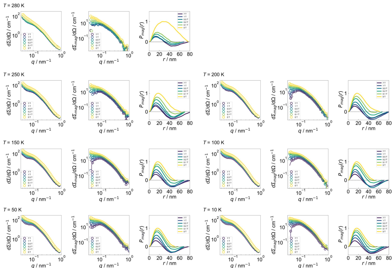
Figure 9 The magnetic field and temperature dependence of the experimental azimuthally averaged (over 2\pi radians) 1D total (nuclear + magnetic) SANS cross sections d\Sigma/d\Omega , the corresponding purely magnetic SANS cross sections d\Sigma_{\text{mag}}/d\Omega and the magnetic distance distribution functions P_{\text{mag}} . The P_{\text{mag}} values were computed numerically via an indirect Fourier transform of the experimental d\Sigma_{\text{mag}}/d\Omega data based on equation (3). The P_{\text{mag}} value at each field has been normalized by the maximum peak intensity value obtained at remanence.
