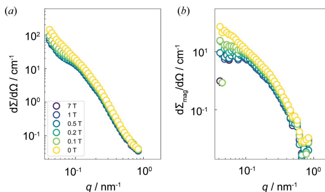
Figure 4 (a) The magnetic field dependence of the azimuthally averaged (over 2\pi radians) total (nuclear + magnetic) SANS cross section d\Sigma/d\Omega at the selected temperature of 280 K. (b) The corresponding purely magnetic SANS cross section d\Sigma_{\text{mag}}/d\Omega (log–log scales).
