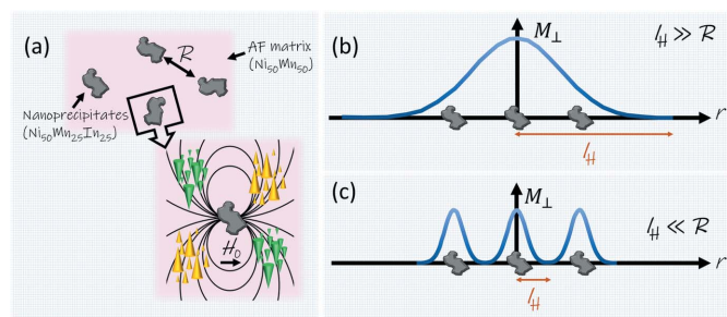
Figure 6 (a) A simplified sketch of the spin-misalignment correlations around defects in an antiferromagnetic matrix. The jump in the magnetization magnitude at the interface between the precipitate and the matrix gives rise to a dipolar stray field (drawn here with spherical symmetry for simplicity), which itself exerts a torque on the matrix spins and in this way produces spin disorder and a concomitant field-dependent contrast for magnetic SANS. R denotes the average distance between defects. Coloured arrows represent the magnetization component \mathbf{M}_{\perp} perpendicular to \mathbf{H}_0 . (b), (c) Illustrations of the magnetization distribution around defects for the cases of l_H \gg R (low field) and l_H \ll R (large field), respectively. Adapted from Kronmüller & Seeger (1961).
