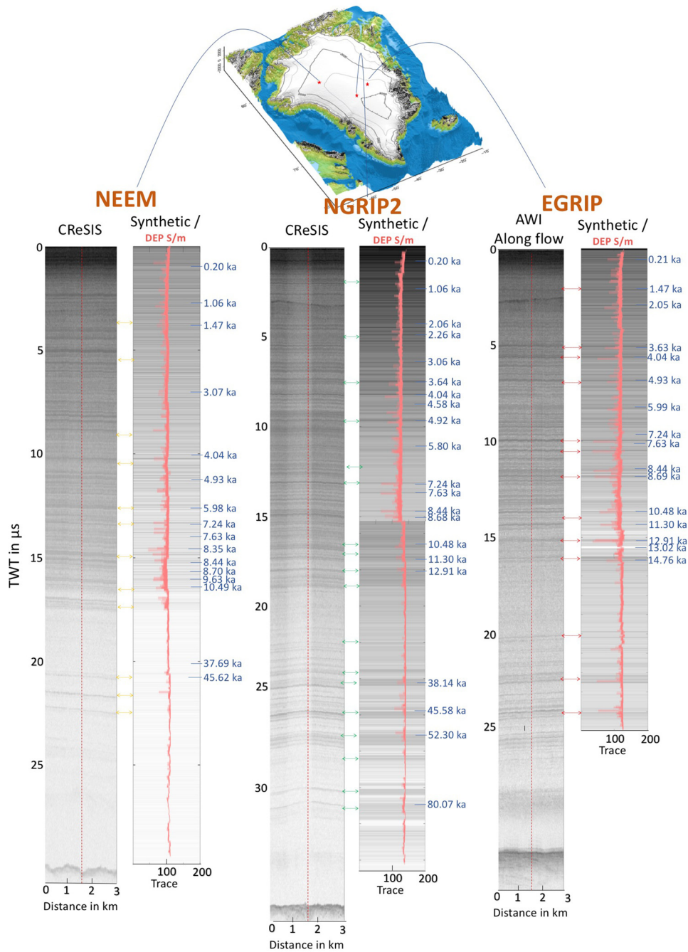
Fig. 3. Z-scopes for synthetic and RES data at the NEEM, NGRIP2 and EGRIP ice cores. The surface reflection of each measured radargram is shifted to time zero. The coloured double arrows indicate the corresponding reflections between synthetic and RES radargrams. The vertical red dashed lines mark the positions of the traces of Figure 2, which correspond to the location of the traces closest to the the borehole locations. The age–depth scale (Rasmussen and others, 2013; Mojtabavi and others, 2020) is based on IRHs in Table 3. The Greenland map is based on the GEBCO (2014) data.
