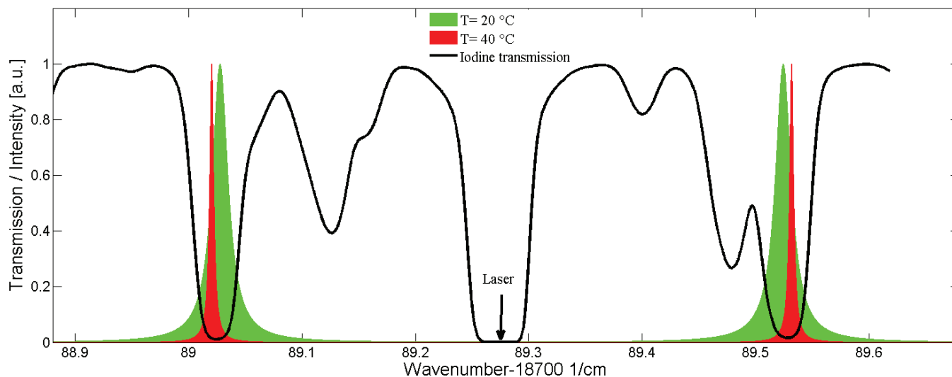
Figure 8. Iodine transmission curve and Brillouin spectra (colored) of water for two temperatures. The Rayleigh spectrum is not shown. Source: DLR.
