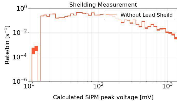
Figure 3: Calculated SiPM Peak Voltage
