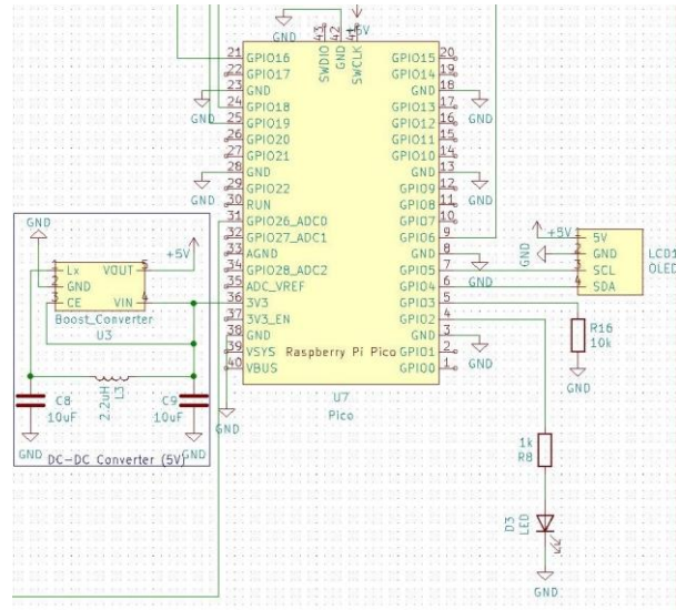
Figure 7: Cosmic Watch Schematic
