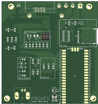
Figure 6: Cosmic Watch 2D View
