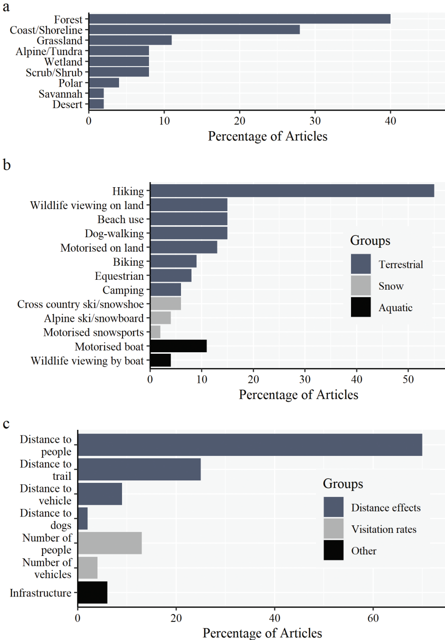
Figure 2. Descriptive statistics of recreation threshold articles. Summary of a ecosystem types b recreation activities and c disturbance variables of articles that identified an effect threshold. Several papers studied more than one ecosystem, recreation activity or disturbance variable, therefore, percentages in one plot sum to greater than 100%. Aquatic recreation only included those water-based activities that effected wildlife on land. Disturbance variable distance to trail included all forms of recreation (e.g. motorised, non-motorised and dogs allowed and not allowed) and infrastructure referred to density of human built strcutres.
