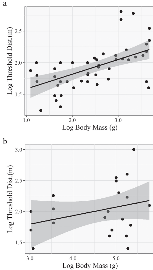
Figure 5. Wildlife body mass as a predictor of effect threshold distance. Regression analysis of body mass as a predictor for a taxon's effect distance threshold for (a) birds and (b) mammals. Black dots indicate individual observations and the shaded area represents the 95% confidence interval.
