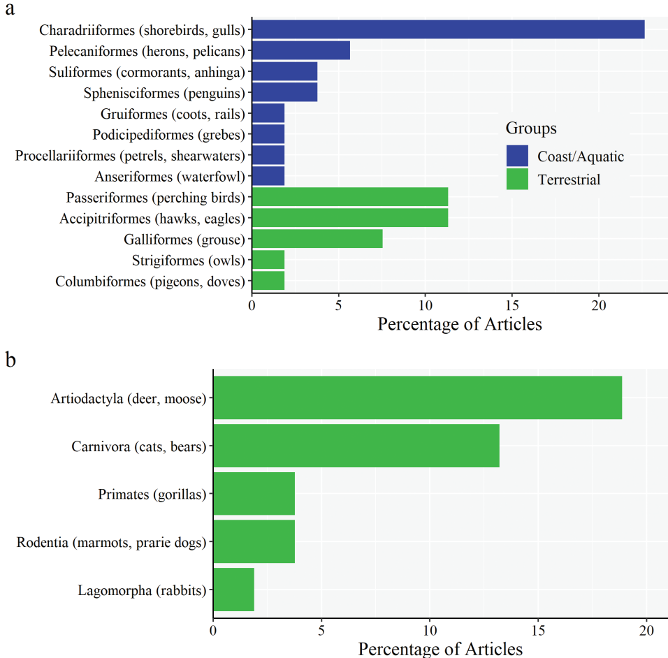
Figure 1. Recreation effect threshold articles by bird and mammal orders (a) bird and (b) mammal orders studied in papers that identified an effect threshold. Several articles contained more than one order, thus, the total number of articles sums to more than all the threshold effects papers.
