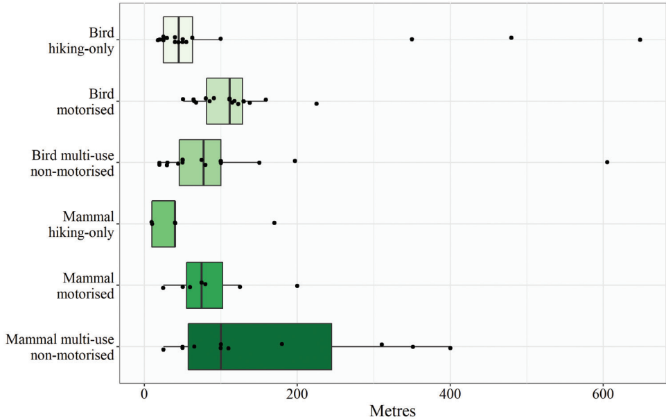
Figure 6. Effect thresholds across groups of recreation activities and taxa. Black dots indicate individual data points. Boxplots indicate median and 25 th and 75 th percentiles. One outlier of 1000 m is not shown for mammal motorised. Whiskers extend to data 1.5 times the interquartile range.
