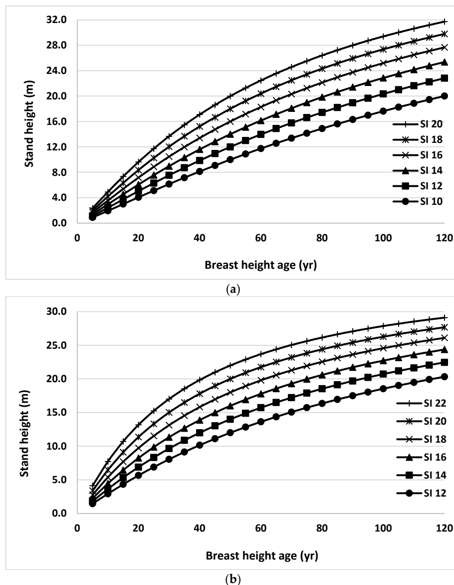
Figure 6. Stand height/site index (SI) profiles generated using Equation (2) for black spruce (a) and trembling aspen (b) trees grown in natural origin mixed stands in Northern Ontario for the range of site productivity.
