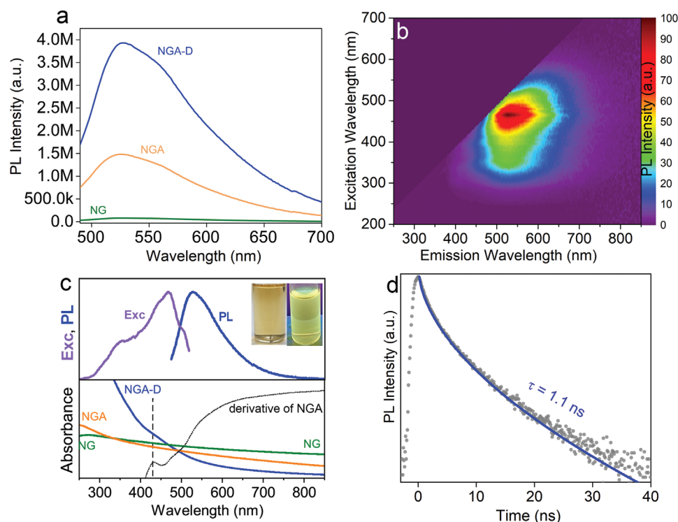
Figure 4. a) Comparison of PL spectra of NG, NGA, and NGA-D ( \lambda_{\text{ex}} = 470 nm, 0.5 mg mL ^{-1} ). b) Excitation-emission color map of NGA-D. c) UV-vis absorption spectra of NG, NGA, and NGA-D (with its derivative), along with the excitation ( \lambda_{\text{ex}} = 467 nm) and PL ( \lambda_{\text{em}} = 527 nm) spectra of NGA-D. The inset in the PL panel shows the aqueous NGA-D dispersion under ambient light and under 365 nm irradiation ( \lambda_{\text{em}} = 527 nm) with corresponding stretched-exponential fit (blue line) for derivation of the PL lifetime. d) Time-resolved PL decay
