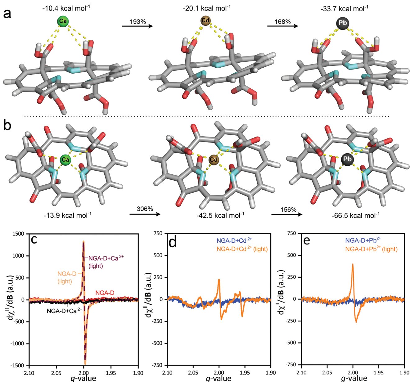
Figure 6. Interaction of three divalent ions ( \text{Ca}^{2+} , \text{Cd}^{2+} , and \text{Pb}^{2+} ) with molecular models of NGA-D, displaying two energetically favorable binding positions comprising a) carboxyl groups only and b) carboxyl groups plus nitrogen atoms, along with their corresponding binding energies (Figures S13 and S14, Supporting Information for further details). X-band CW-EPR and CW-LEPR spectra of NGA-D dispersed in \text{H}_2\text{O} and measured in frozen matrix ( T = 80\text{ K} ) of c) pure NGA-D recorded under dark conditions (red line) and under UV irradiation (orange line) and NGA-D with adsorbed \text{Ca}^{2+} cations recorded under dark conditions (black line) and under UV irradiation (purple dashed line). d) NGA-D with adsorbed \text{Cd}^{2+} cations recorded under dark conditions (blue line) and under UV irradiation (orange line). e) NGA-D with adsorbed \text{Pb}^{2+} cations recorded under dark conditions (blue line) and under UV irradiation (orange line).
