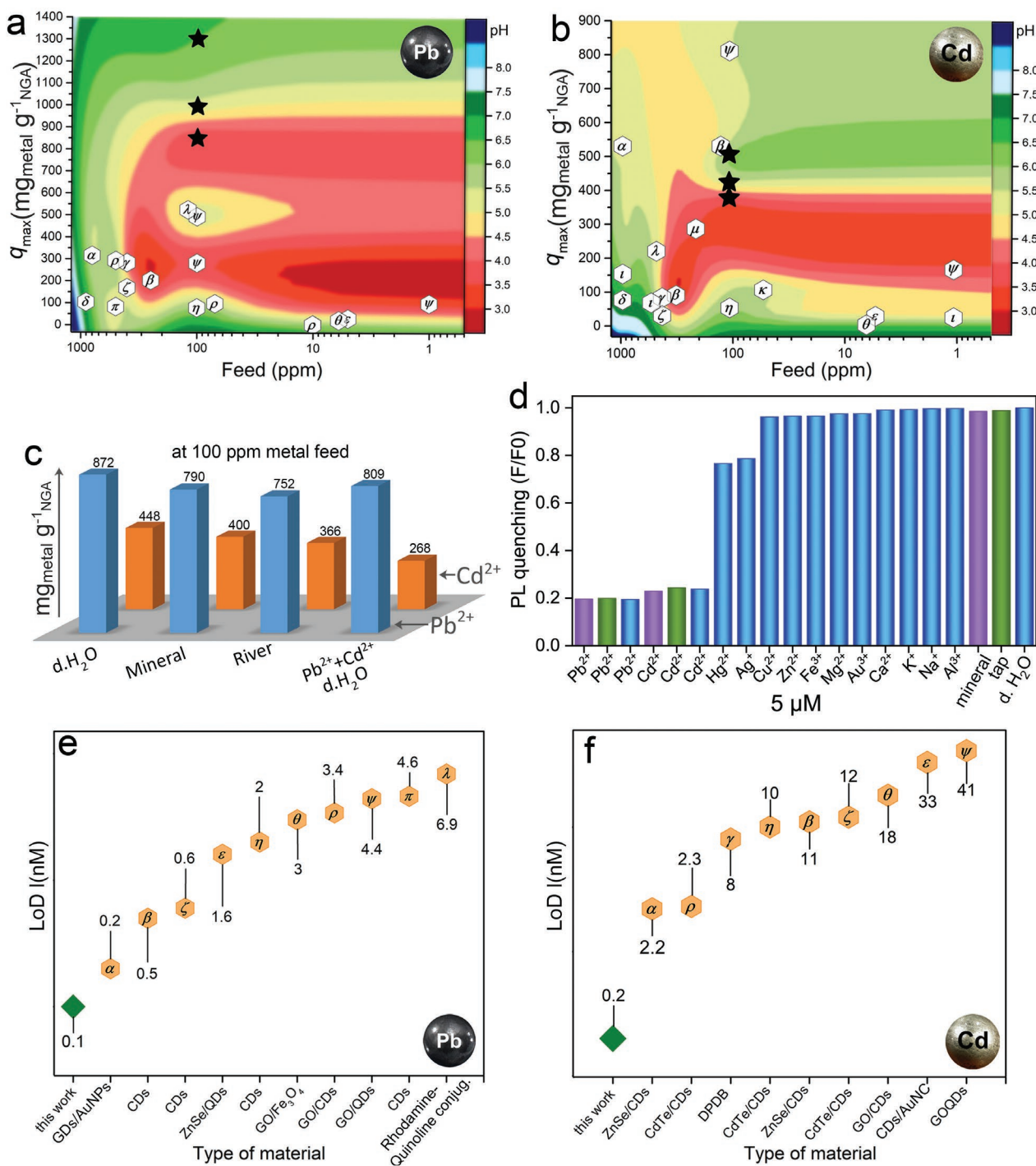
Figure 5. a,b) Comparative graph showing the adsorption capacities ( q_{max} ) for Pb 2+ and Cd 2+ for NGA (star symbols) and for previously reported sorbents at various metal feeds and pH values: ( \alpha ) MOF-808(Zr) modified with EDTA, [10] ( \beta ) GO, [68] ( \gamma ) GO/polymer hydrogel, [69] ( \delta ) carbon nanotube sheets, [70] ( \epsilon ) GO, amino-modified and decorated with Fe 3 O 4 nanoparticles, [71] ( \zeta ) copolymer modified Fe 3 O 4 nanoparticles, [72] ( \eta ) silica gel modified with nitrilotriacetic acid, [73] ( \theta ) GO decorated by iron-based nanoparticles, [74] ( i ) GO, [75] ( \kappa ) GO, [76] ( \lambda ) 2D Ca 2+ -MOF, [17] ( \mu ) FJI-H9 MOF modified with amino groups, [77] ( \pi ) \alpha -FeOOH, [78] ( \rho ) LDH modified with MoS 4 2- , [79] ( \psi ) graphene acid. [12] c) Adsorption capacities at pH = 3.5 for Pb 2+ and Cd 2+ in distilled, mineral, and river water, as well in combined Pb 2+ and Cd 2+ solutions in distilled water. In all experiments, the initial metal feed was 100 ppm. d) Comparison of fluorescence quenching of NGA-D induced by Pb 2+ , Cd 2+ , and other metal ions at 5 \mu M concentration in ultra-pure water (blue), tap water (green), and mineral water (purple). e) Comparative graph showing the LoD values for Pb 2+ for NGA-D and from the state-of-the-art material sensors. ( \alpha ) GQDs modified with AuNPs, [21] ( \beta ) CDs, [19] ( \zeta ) CDs, [29] ( \epsilon ) ZnSe QDs, [25] ( \eta ) CDs, [45] ( \theta ) GO dots modified with Fe 3 O 4 , [80] ( \rho ) GO combined with CDs, [81] ( \psi ) GO combined with QDs, [38] ( \pi ) CDs, [30] ( \lambda ) Rhodamine-Quinoline Conjugates, [82] f) Comparative graph showing the limit of detection for Cd 2+ for NGA-D and for top-rated results from literature. ( \alpha ) ZnSe/CDs, [25] ( \rho ) CdTe QDs, [26] ( \gamma ) DPDB ligand, [83] ( \eta ) CdTe QDs, [84] ( \beta ) ZnSe/CdS, [24] ( \zeta ) CdTe QDs, [85] ( \theta ) GO combined with CDs, [86] ( \epsilon ) CDs modified with gold nanoclusters [87] and ( \psi ) GOQD. [38]
