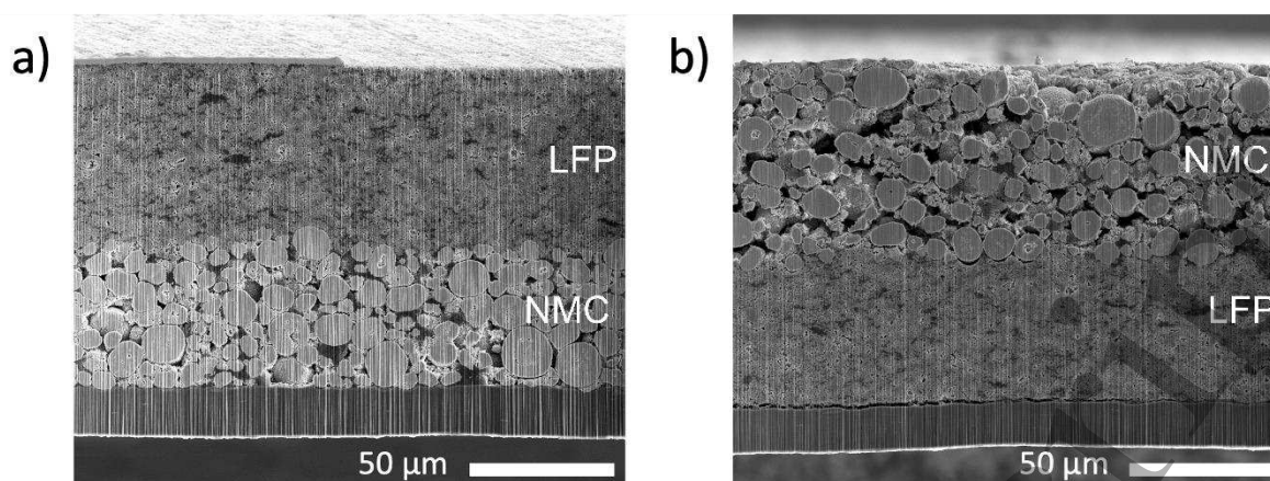
Figure 2. SEM-FIB cross section images of a) NMC/LFP and b) LFP/NMC bilayer electrodes produced by multi-pass doctor blade coating.
