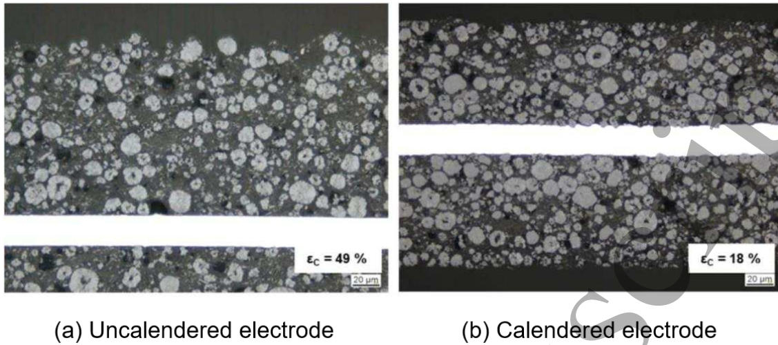
Figure 1. SEM images of electrode deformation before/after calendaring, showing the active material (AM) particle phase and carbon binder domain (CBD) phase [1]
