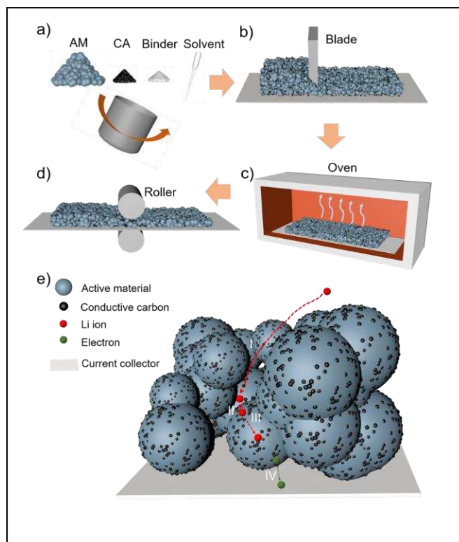
Figure 1. Slurry cast processing a-d; a) mixing of active material (AM), conductive additive (CA), binder and solvent; b) coating via a doctor blade on a metallic foil; c) drying; d) calendaring; e) schematic illustration of the transport of lithium ions and electrons, I) lithium ions diffuse in the bulk electrolyte, II) charge transfer at the electrode/electrolyte interface, III) solid-state diffusion of lithium ions within active material particles, IV) electrons transfer from conductive carbon network to the current collector
