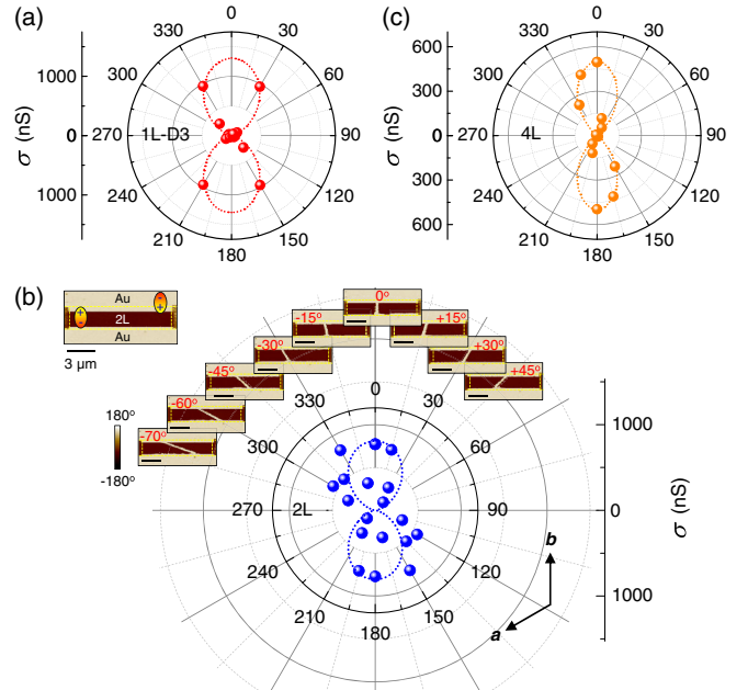
FIG. 3. Polar plots of \sigma of (a) 1L \text{ReS}_2 at V_{\text{bg}} = 40 V, (b) a 2L \text{ReS}_2 at V_{\text{bg}} = -40 V, and (c) a 4L \text{ReS}_2 at V_{\text{bg}} = 10 V. The dashed lines serve as a guide to the eye. Insets in (b): PFM phase images of the corresponding P_{\text{down}} nanowires. The top left image corresponds to the initial uniform P_{\text{up}} domain before the nanowire patterning. All scale bars are 3 \mu\text{m} .
