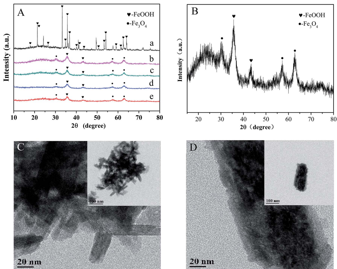
Fig. 1 (A) XRD patterns: (a) only FeOOH, (b) 10% Co-doped \text{Fe}_3\text{O}_4@/\text{FeOOH} , (c) 5% Co-doped \text{Fe}_3\text{O}_4@/\text{FeOOH} , (d) 1% Co-doped \text{Fe}_3\text{O}_4@/\text{FeOOH} , (e) \text{Fe}_3\text{O}_4@/\text{FeOOH} . (B) XRD pattern of 10% Co-doped \text{Fe}_3\text{O}_4@/\text{FeOOH} . (C) and (D) TEM images of 10% Co-doped \text{Fe}_3\text{O}_4@/\text{FeOOH} .
