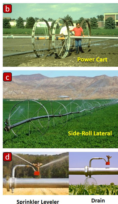
Figure 12.4. Side-roll sprinkler system and components. (The plan view shown in drawing a is adapted from Turner and Anderson, 1980. Picture c is courtesy of Rain for Rent and picture d is courtesy of Wade Rain, Inc.).
