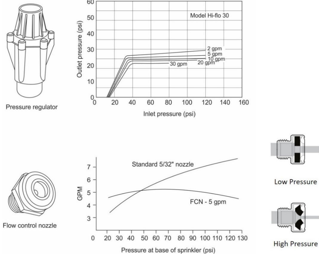
Figure 11.10. Performance of a pressure regulator at several flow rates, and a flow control nozzle (courtesy of Nelson Irrigation Corp.).
