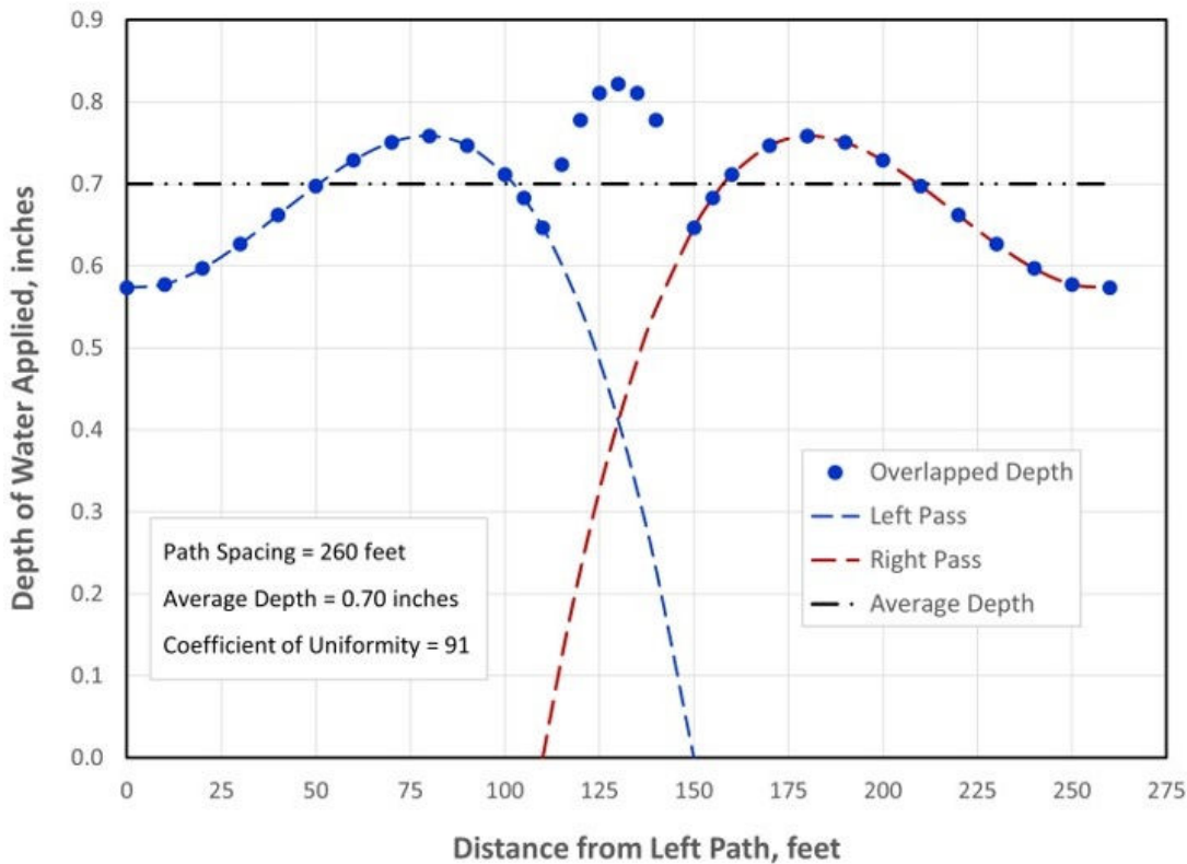
Figure 12.19. Distribution of water from a single pass of a traveler for three types of gun settings, and the overlapped patterns for the medium size gun with a central angle of 270°. Based on data from Ge et al. (2018) and Prado and Colombo (2020).
