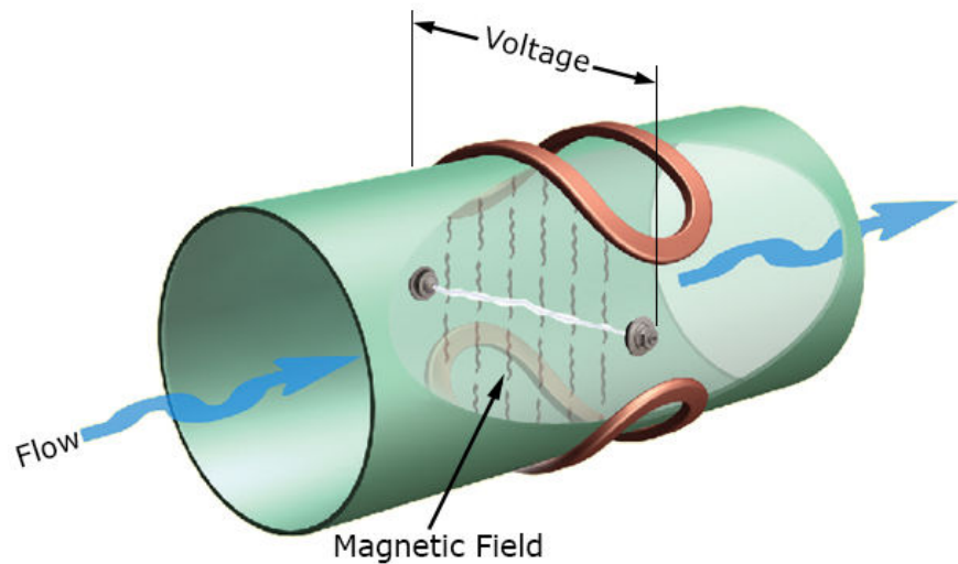
Figure 3.14. In-line magnetic flowmeter. (Modification of diagram provided courtesy of McCrometer Corporation.)
