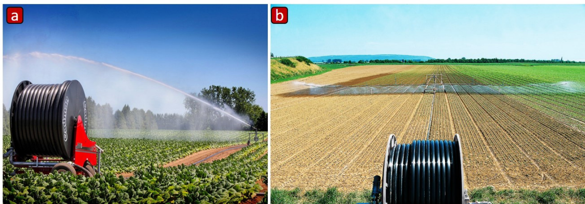
Figure 12.17. Hard-hose traveler diagram with photo of a traveler with a gun (photo a is courtesy of Cadman Power Equipment) and with large boom (photo b is courtesy of Bauer Group).
