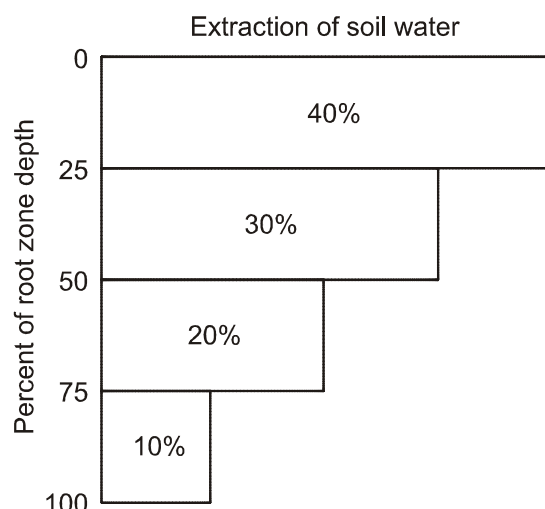
Figure 6.4. Average water extraction pattern from the plant root zone, the 4-3-2-1 rule.
