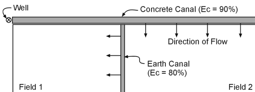
Figure 5.12. Example of a farm layout with seepage losses between the source of the water and delivery to the field.
