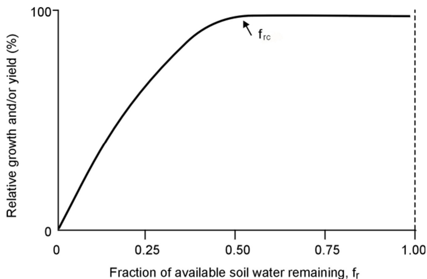
Figure 6.2. Relationship between available water remaining and yield (adopted from Stegman, 1983).
