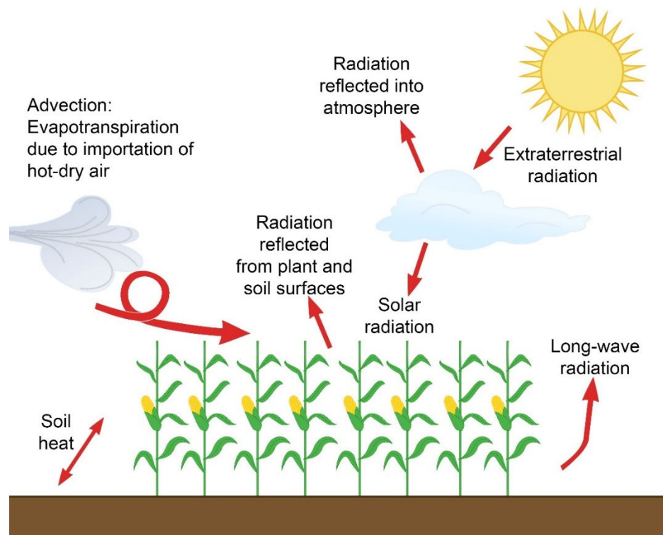
Figure 4.5. Diagram of energy sources for evapotranspiration.
