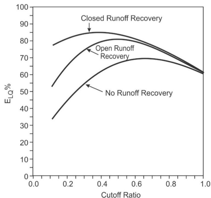
Figure 10.15. E_{LQ} vs. cutoff ratio for sloping furrows with medium textured soils (silt, silt loams, loams and sandy clays). Assumes advance time exceeds recession time.
