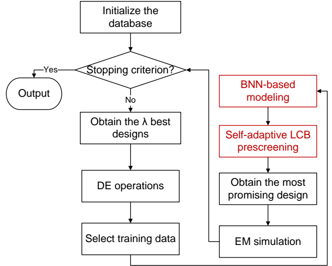
Figure 1. Flow diagram of SB-SADEA
