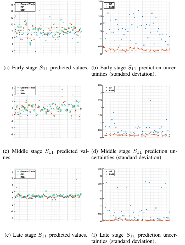
Figure 3. GP and BNN predicted values and prediction uncertainty during early, middle and late stage of the optimization (ground truth is from EM simulations).
