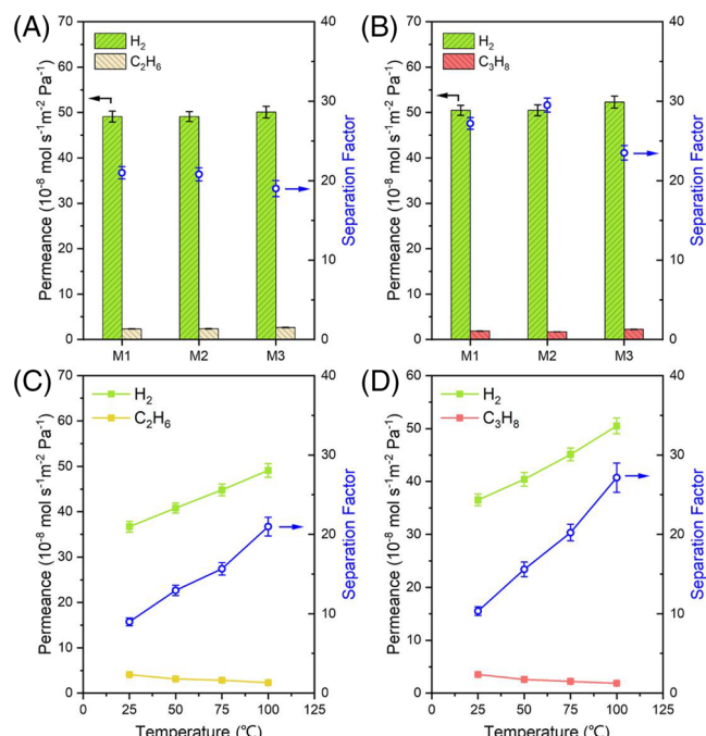
FIGURE 14 H 2 , C 2 H 6 , and C 3 H 8 permeances and separation factors for mixture gases (50%:50% in volume) of (A) H 2 /C 2 H 6 and (B) H 2 /C 3 H 8 on thin membranes of SSZ-13 zeolite (M1, M2, and M3 were synthesized by the same method, thicknesses of ~500 nm) tested at 120 kPa (feed pressure) and 100°C. Gas permeances and separation factors for mixture (C) H 2 /C 2 H 6 and (D) H 2 /C 3 H 8 gases at different temperatures tested at 120 kPa (feed pressure)
