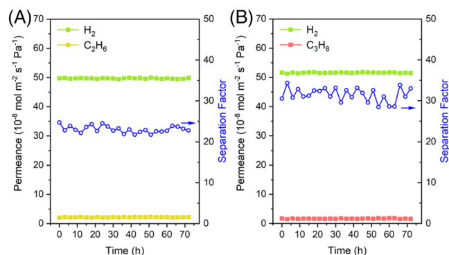
FIGURE 16 H 2 , C 2 H 6 , and C 3 H 8 permeances, and separation factors as a function of operation time for mixture gases (50%:50% in volume) of (A) H 2 /C 2 H 6 and (B) H 2 /C 3 H 8 on the thin SSZ-13 zeolite membrane measured at 120 kPa (feed pressure) and 100°C
