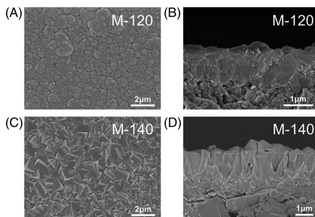
FIGURE 8 SEM images from top (A, C) and side (B, D) views for the membranes of SSZ-13 zeolite synthesized in the gels with dual templates of TMAdaOH:TEAOH = 1.5:0.5 at varied crystallization temperatures ( 120^\circ\text{C} (A, B), 140^\circ\text{C} (C, D)); the resultant membranes are labeled as M-120, M-140 for 24 h
