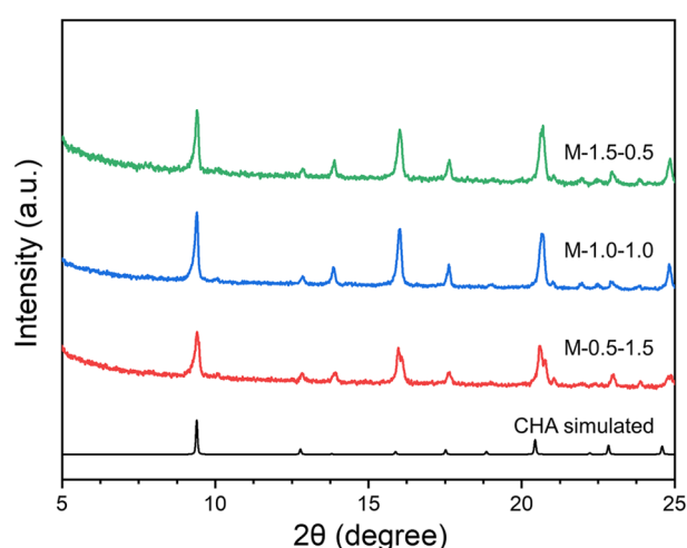
FIGURE 6 XRD patterns of SSZ-13 membranes synthesized in dual-template gels with varied TMAdaOH:TEAOH ratios at 160°C for 24 h
