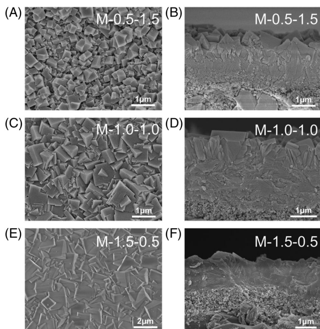
FIGURE 7 SEM images from top (A, C, E) and side (B, D, F) views for SSZ-13 membranes synthesized in dual-template gels with varied TMAdaOH:TEAOH ratios of x:y = 0.5:1.5 (A, B), 1.0:1.0 (C, D), 1.5:0.5 (E, F) at 160^\circ\text{C} for 24 h
